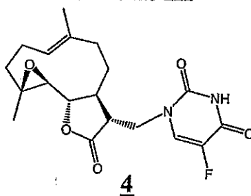
5-Fluorouracil-Parthenolide Codrug
