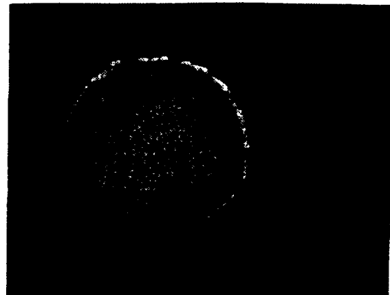
(100 ThO 2 )
