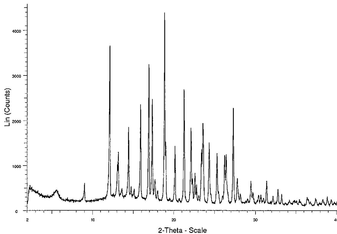
Fig 1 Free molecule (no salt) Example 1 PXRD
