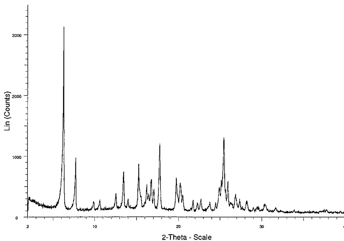
Figure 7 Example 1 besylate salt PXRD
