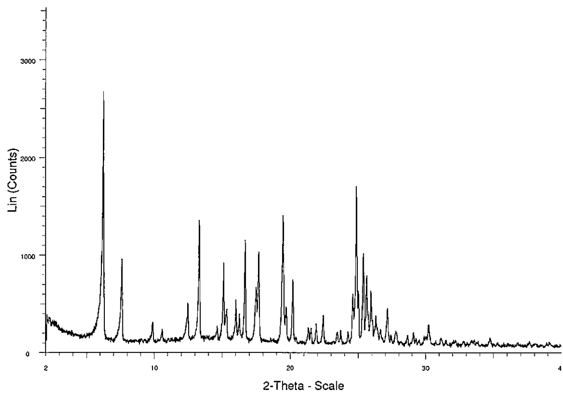
Figure 4 Example 1 tosylate salt PXRD
