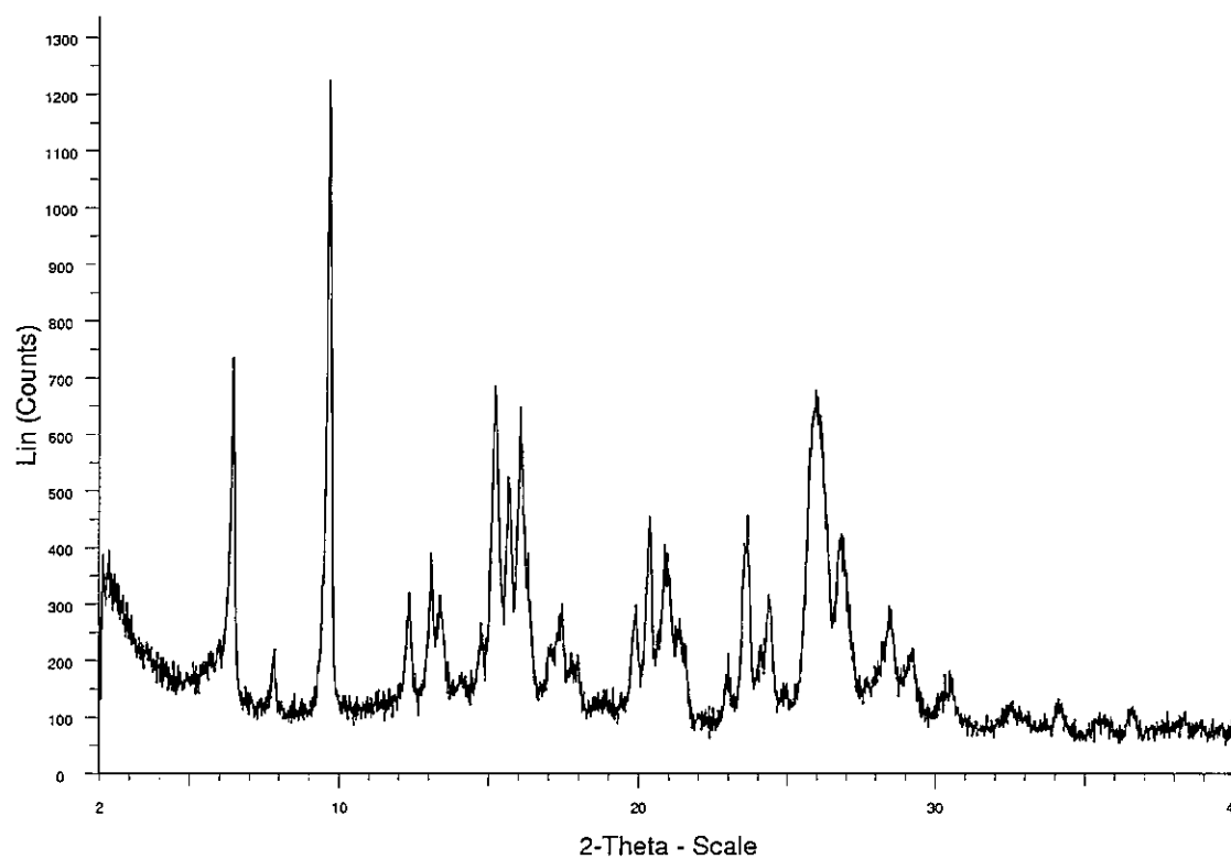
Figure 12 Example 1 Napadysilate salt PXRD
