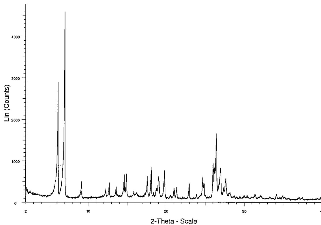
Figure 5 Example 1 hydrochloride salt PXRD
