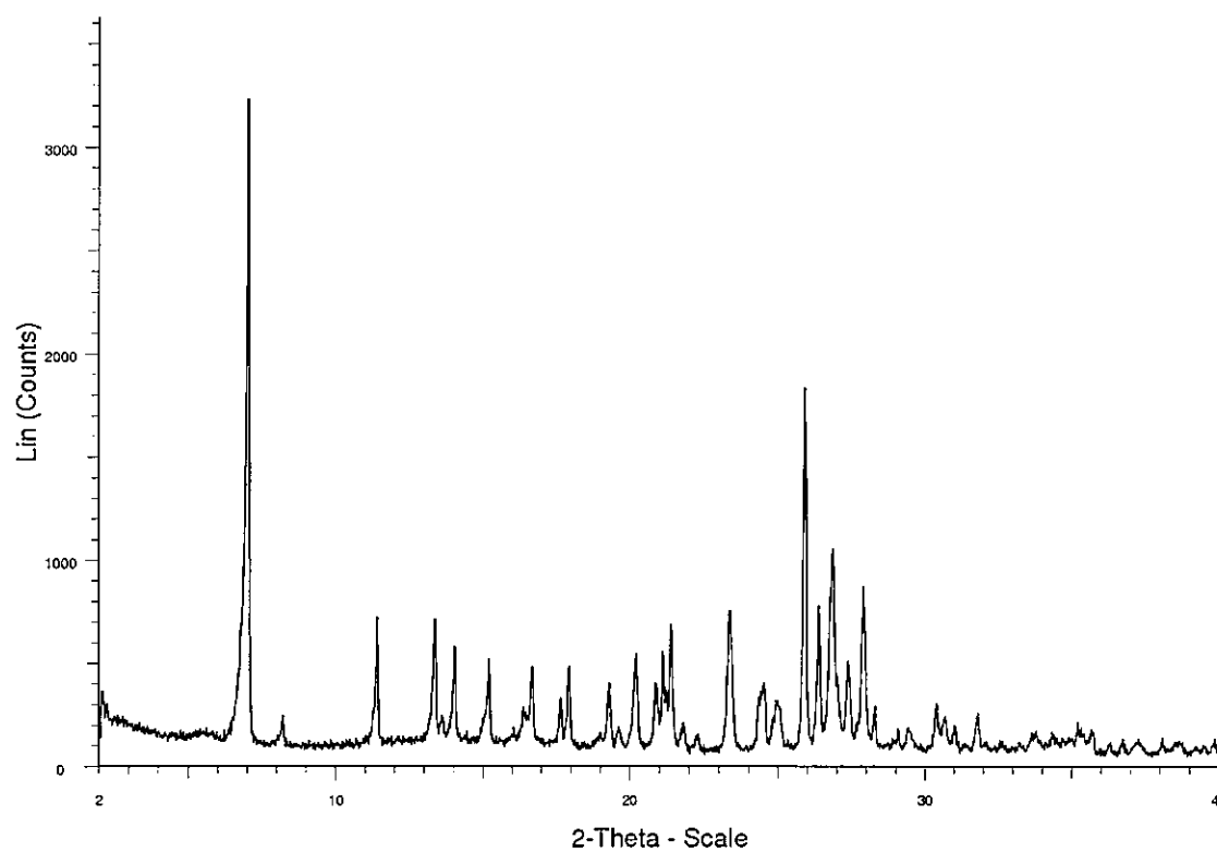
Figure 9 Example 1 hydrobromide salt PXRD
