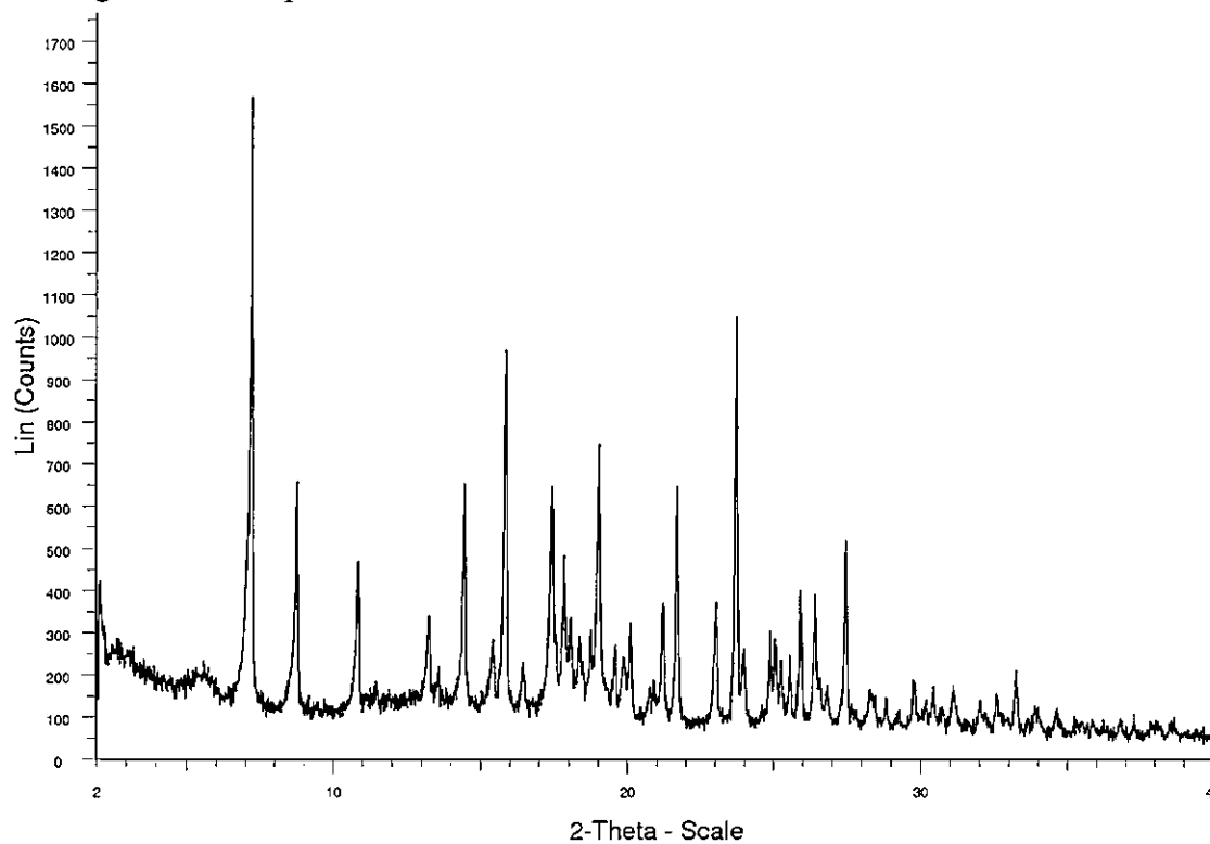
Figure 11 Example 1 Fumarate salt PXRD
