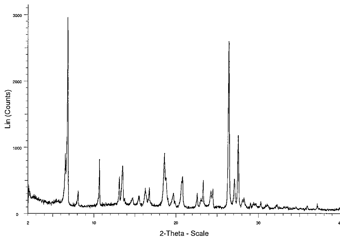
Figure 6 Example 1 sulphate salt PXRD
