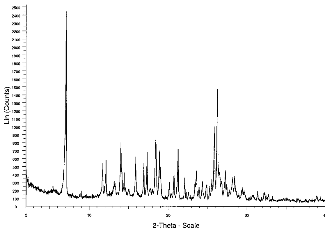
Fig 2 Example 1 nitrate salt PXRD
