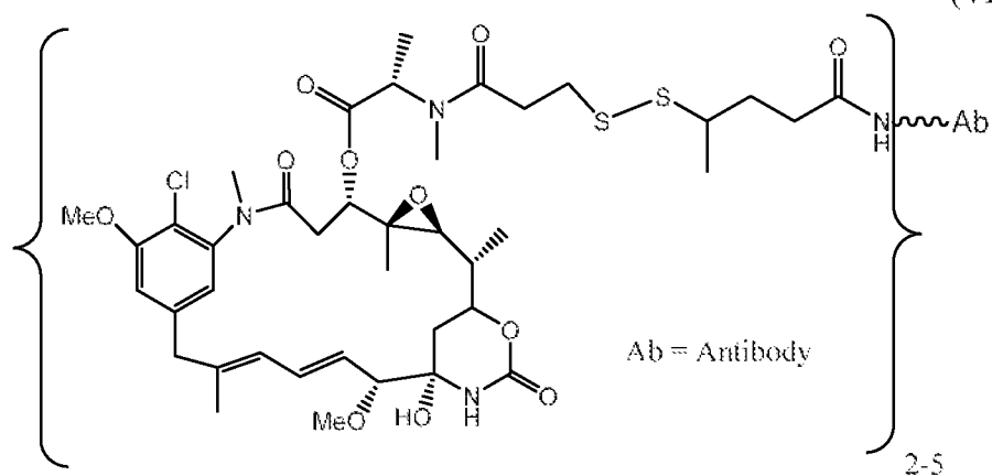
Ab-SPP-DM1
