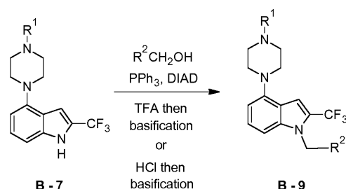
Reaction Scheme 6.
