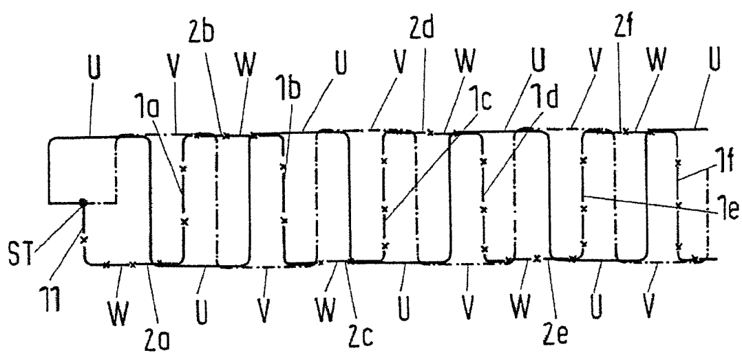
Fig.3 (prior art)
