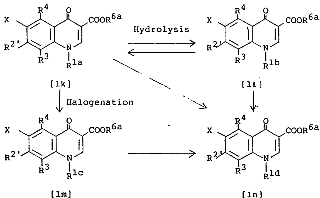
[Reaction scheme-XVI]
