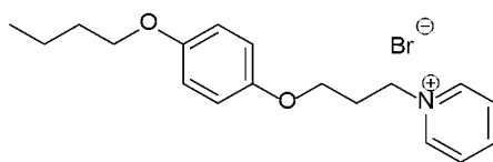
Compound 44A
