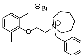
Compound 1A
