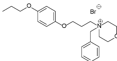
Compound 47A
