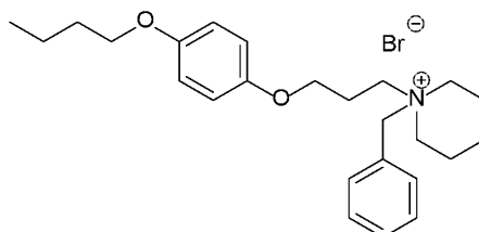
Compound 38A
