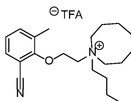
Compound 33A
