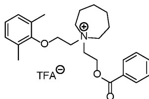
Compound 35A
