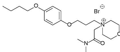
Compound 54A
