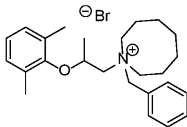
Compound 34A
