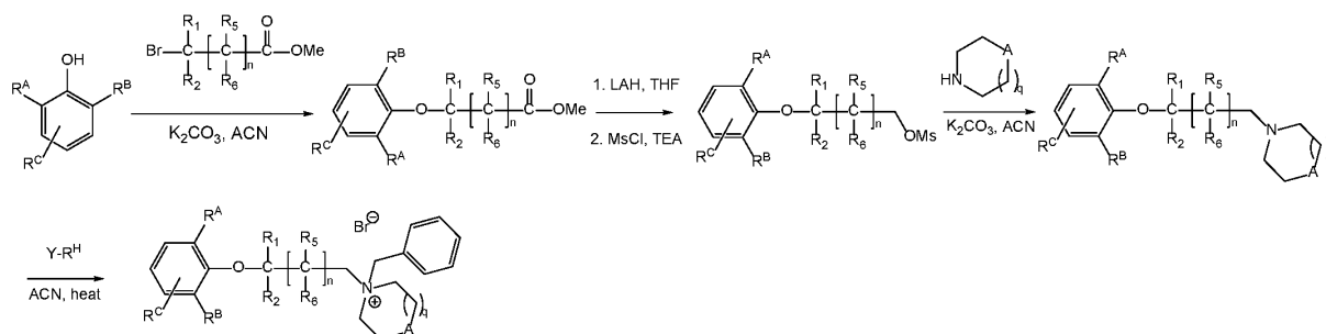
Scheme D:
