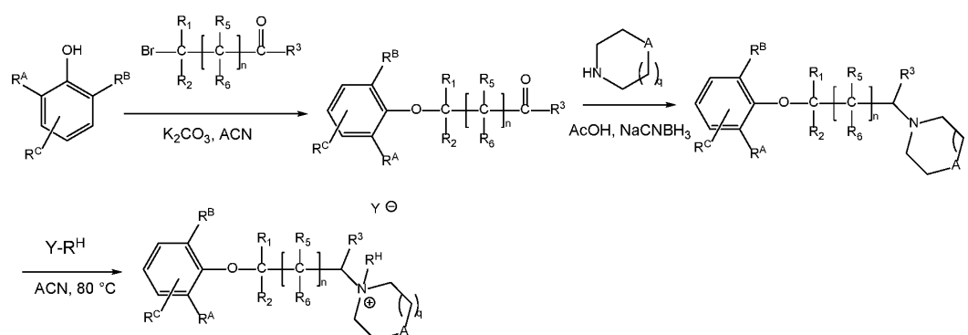
Scheme E:
