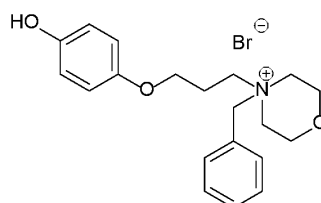
Compound 53A
