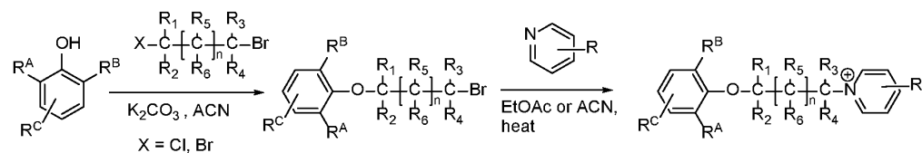
Scheme C:
