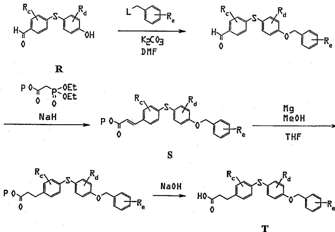
Scheme 6
