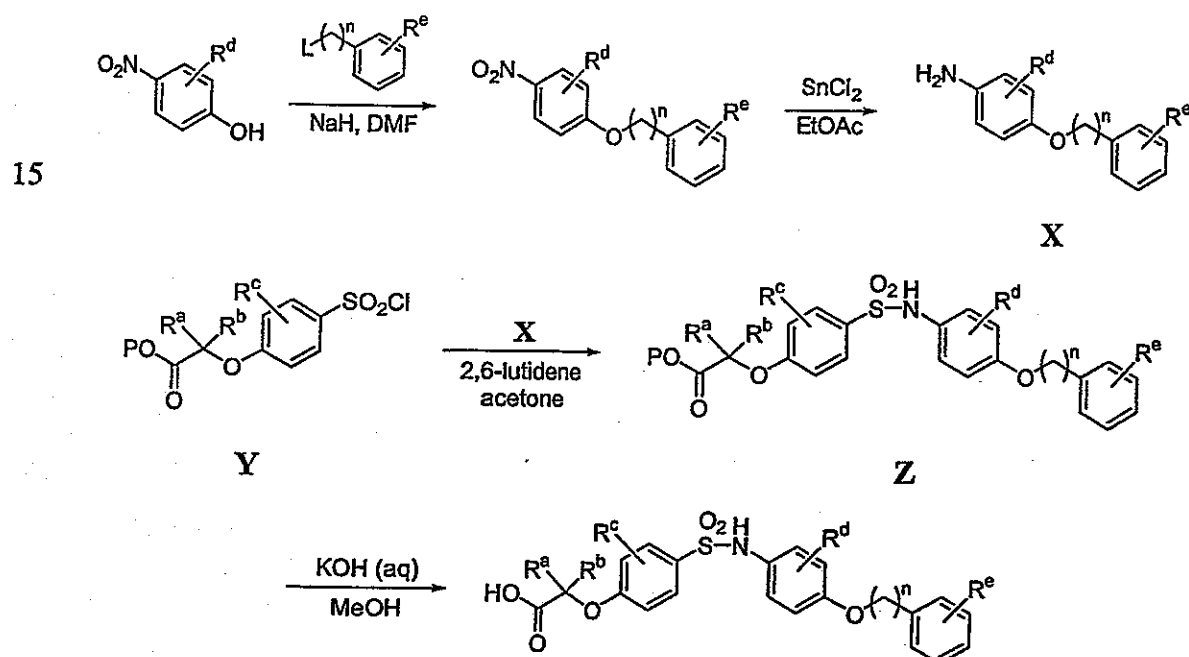
Scheme 8
