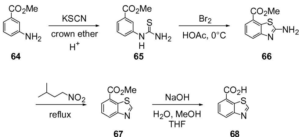
Scheme 9: Synthesis of benzothiazole-carboxylic acid derivatives
