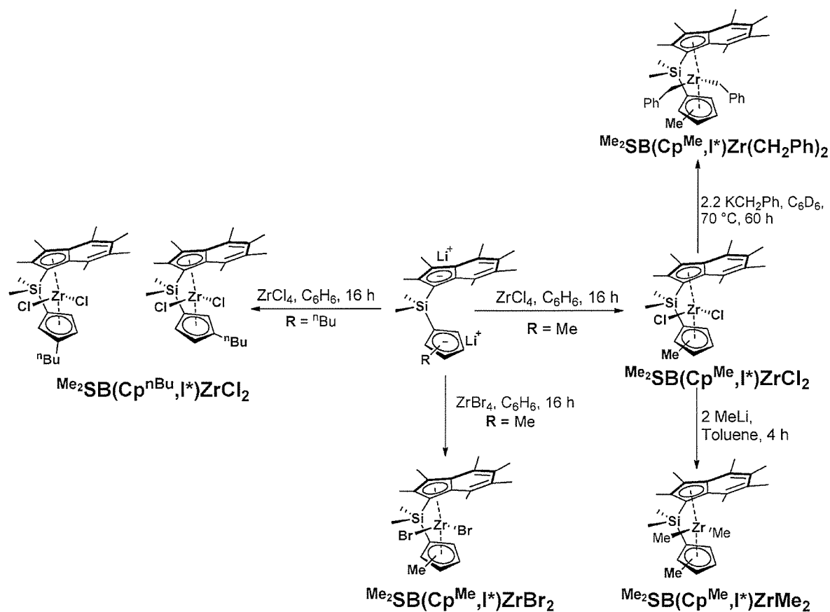
Scheme 1b - Synthesis of various unsymmetrical \text{Me}_2\text{SB}(\text{Cp}^{\text{R}},\text{I}^*)\text{ZrCl}_2 compounds of the invention
