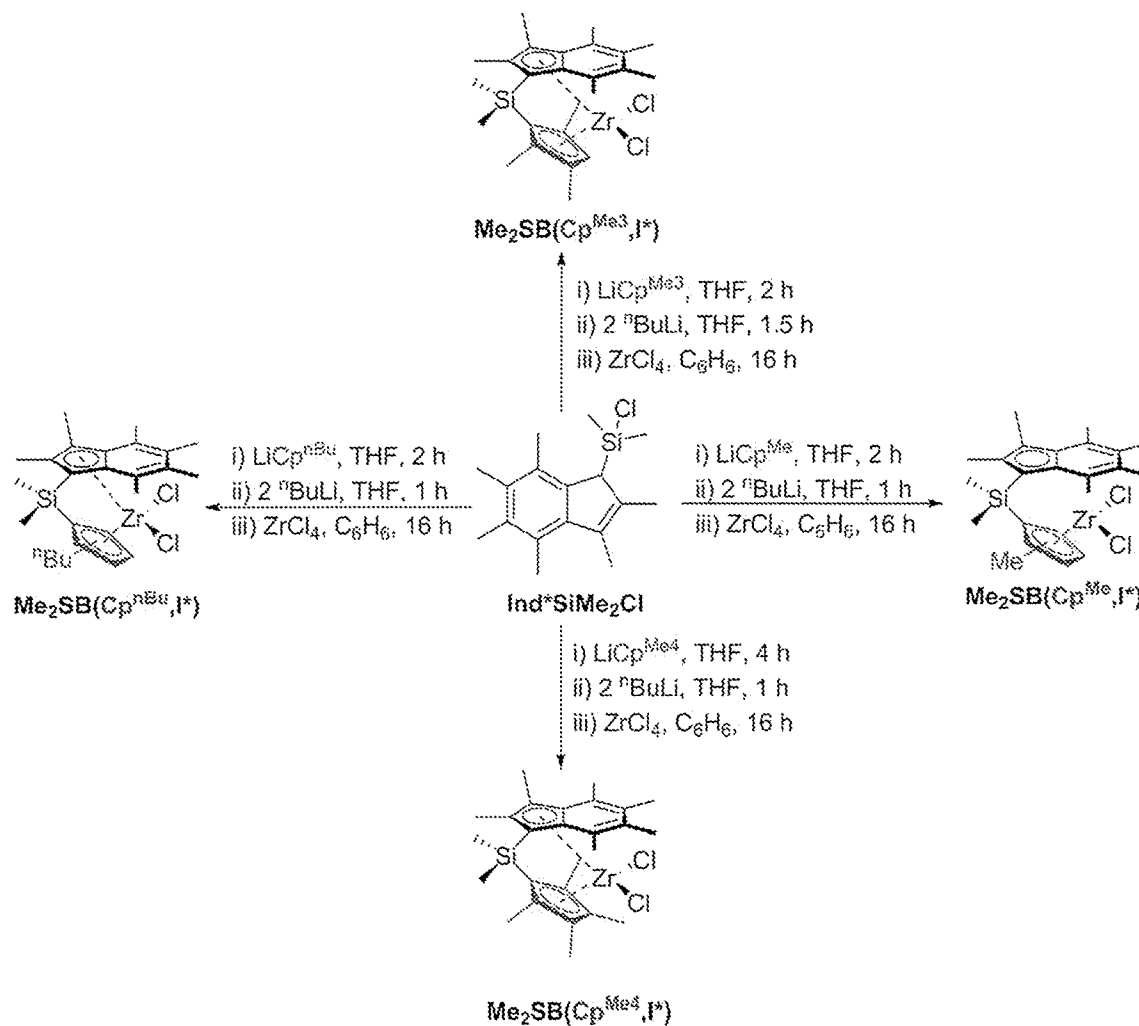
Scheme 1a - Synthesis of various unsymmetrical \text{Me}_2\text{SB}(\text{Cp}^{\text{R}}, \text{I}^*)\text{ZrCl}_2 compounds of the invention
