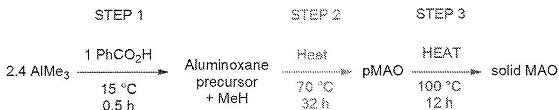
Scheme 2 - Synthesis of solid MAO (1.2/70,32/100,12)
