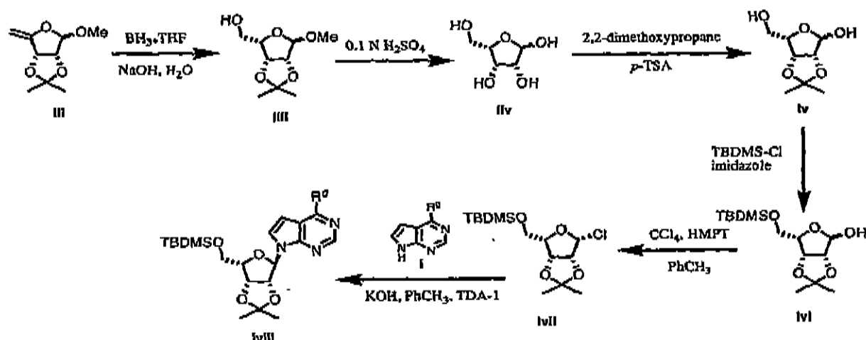
Scheme 10: Synthesis of ((2 S ,3 S ,4 R ,5 R )-5-(4-(alkylamino)-7 H -pyrrolo[2,3- d ]pyrimidin-7-yl)-3,4-dihydroxy-tetrahydrofuran-2-yl)methyl sulfamates
