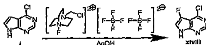
Scheme 8: Synthesis of 5-fluoro pyrrolo[2,3- d ]pyrimidines
