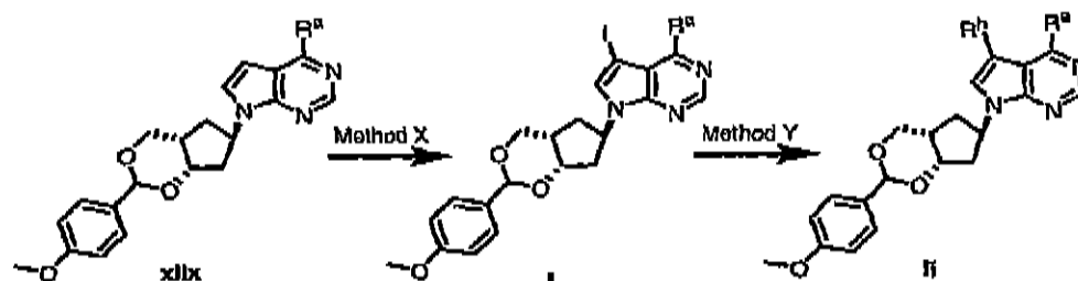
Scheme 9: Alternate route to of 4,5-disubstituted ((1 S ,2 S ,4 R )-2-hydroxy-4-(7 H -pyrrolo[2,3- d ]pyrimidin-7-yl)cyclopentyl)methyl sulfamates
