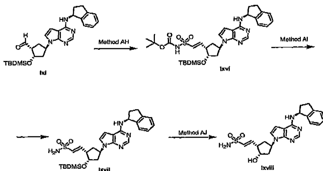
Scheme 12: Synthesis of ( E )-2-((1 S ,2 S ,4 R )-4-[4-[(1 S )-2,3-dihydro-1 H -inden-1-ylamino]-7 H -pyrrolo[2,3- d ]pyrimidin-7-yl]-2-hydroxycyclopentyl)ethylenesulfonamide
