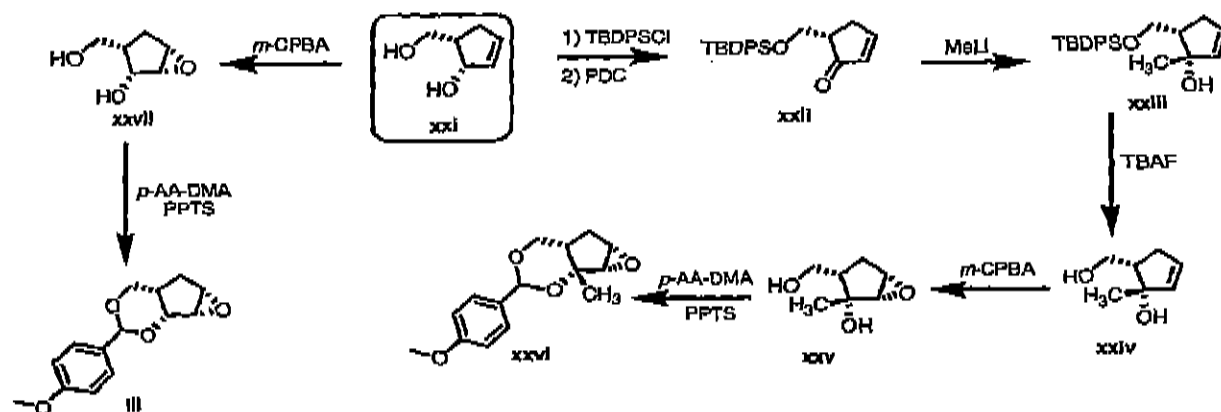
Scheme 3: Synthesis of substituted epoxides
