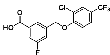
1-65
