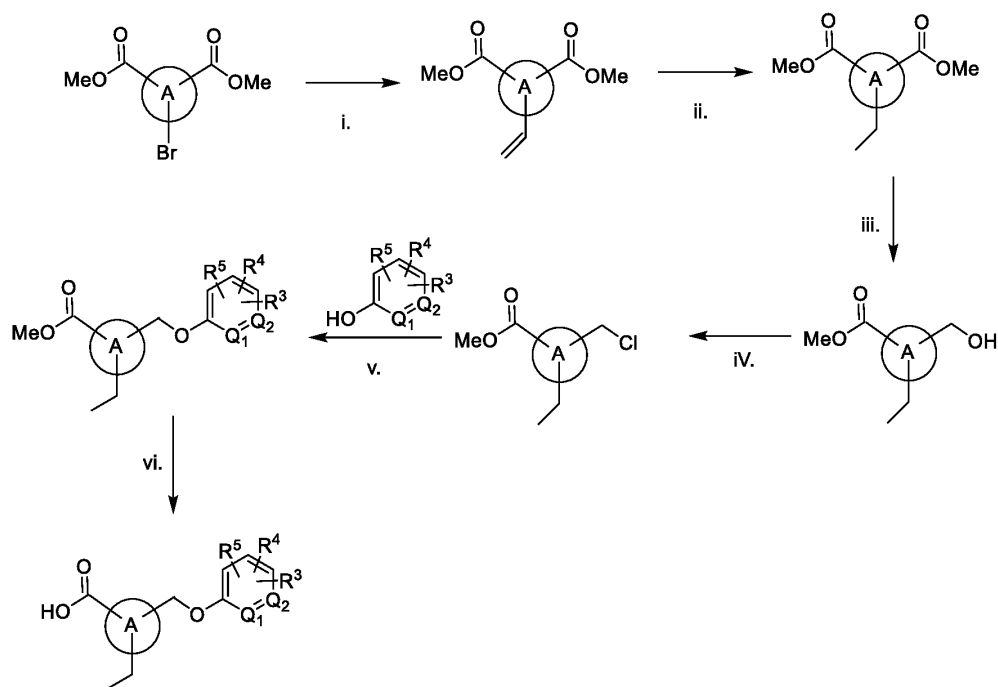
Scheme 37
