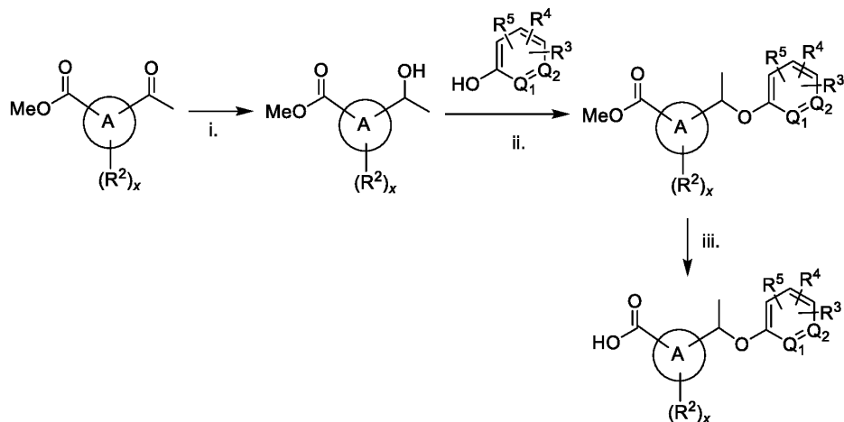
Scheme 62
