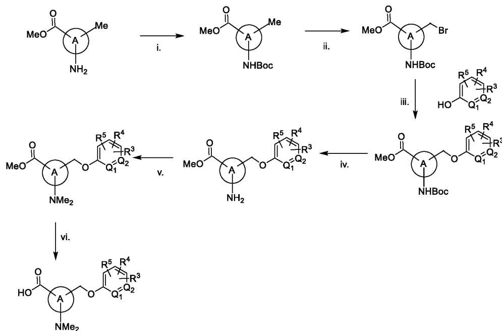
Scheme 38
