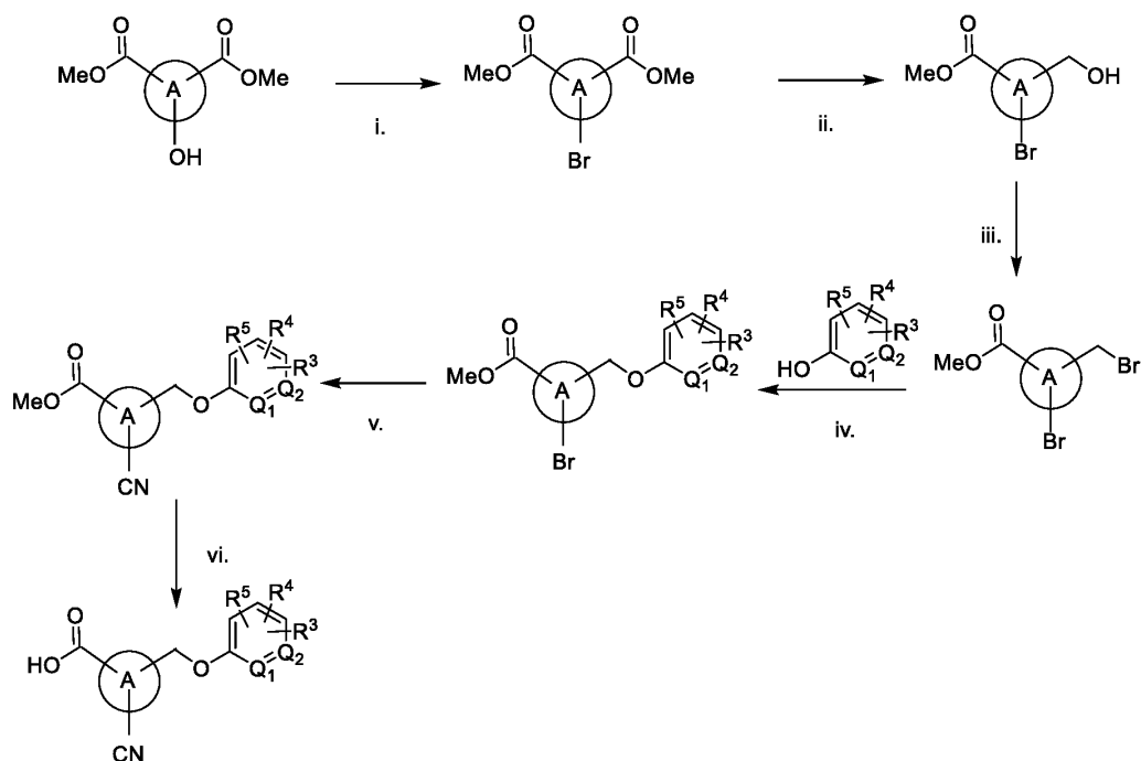
Scheme 43
