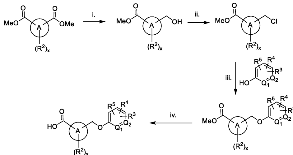
Scheme 31
