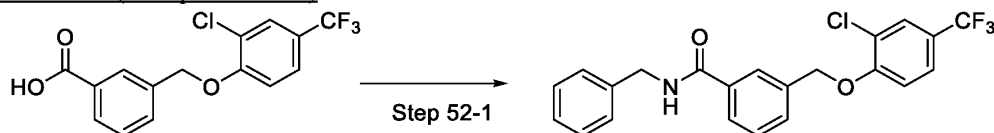
Compound 1-55
