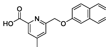
Compound 41-1
