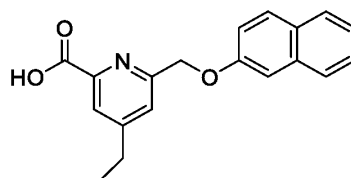
Compound 42-1
