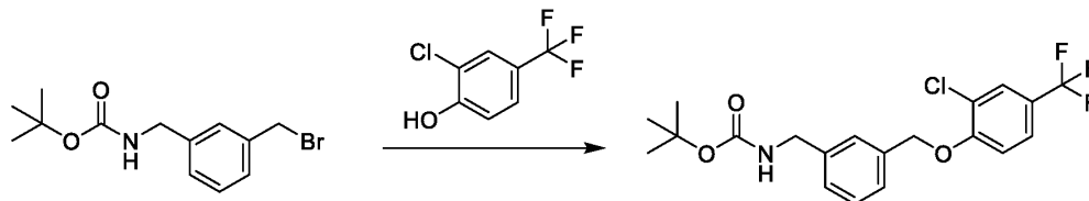
INT 63-1
