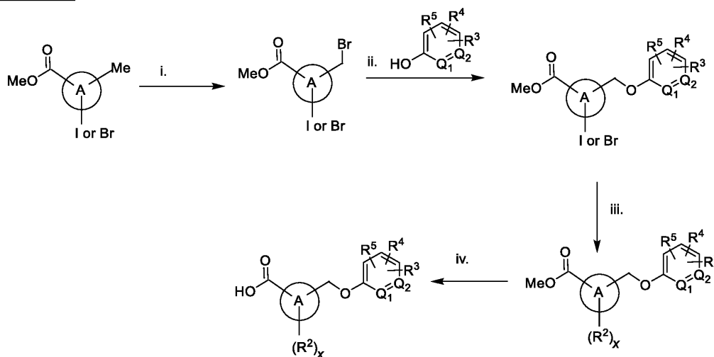
Scheme 8
