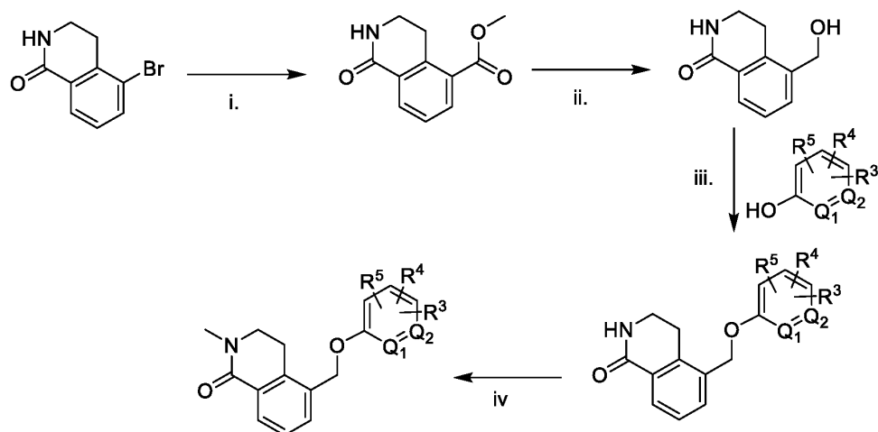
Scheme 58
