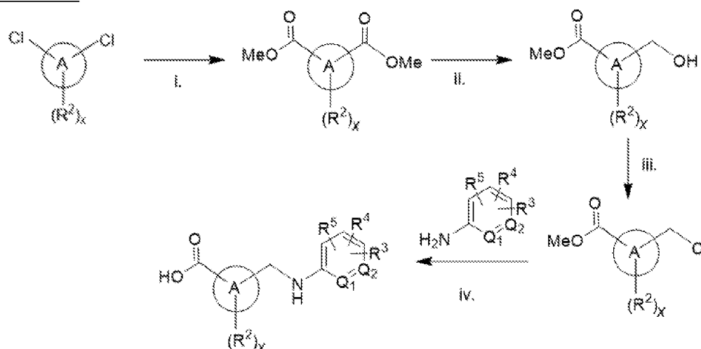
Scheme 57
