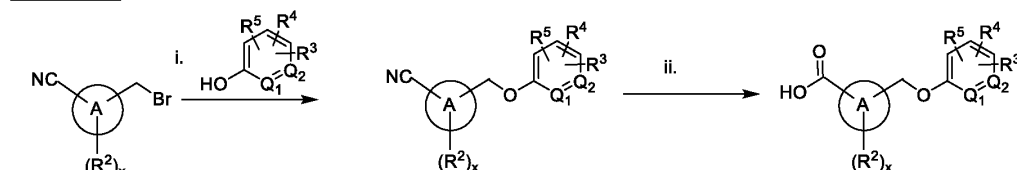
Scheme 3
