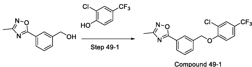
Compound 49-1
