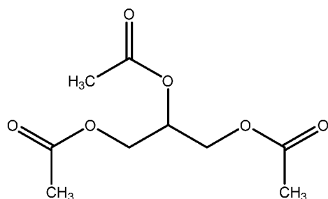
Triacetin
