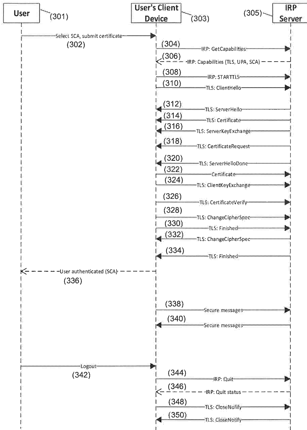
SCA - TLS 1.2 with Mutual Authentication
