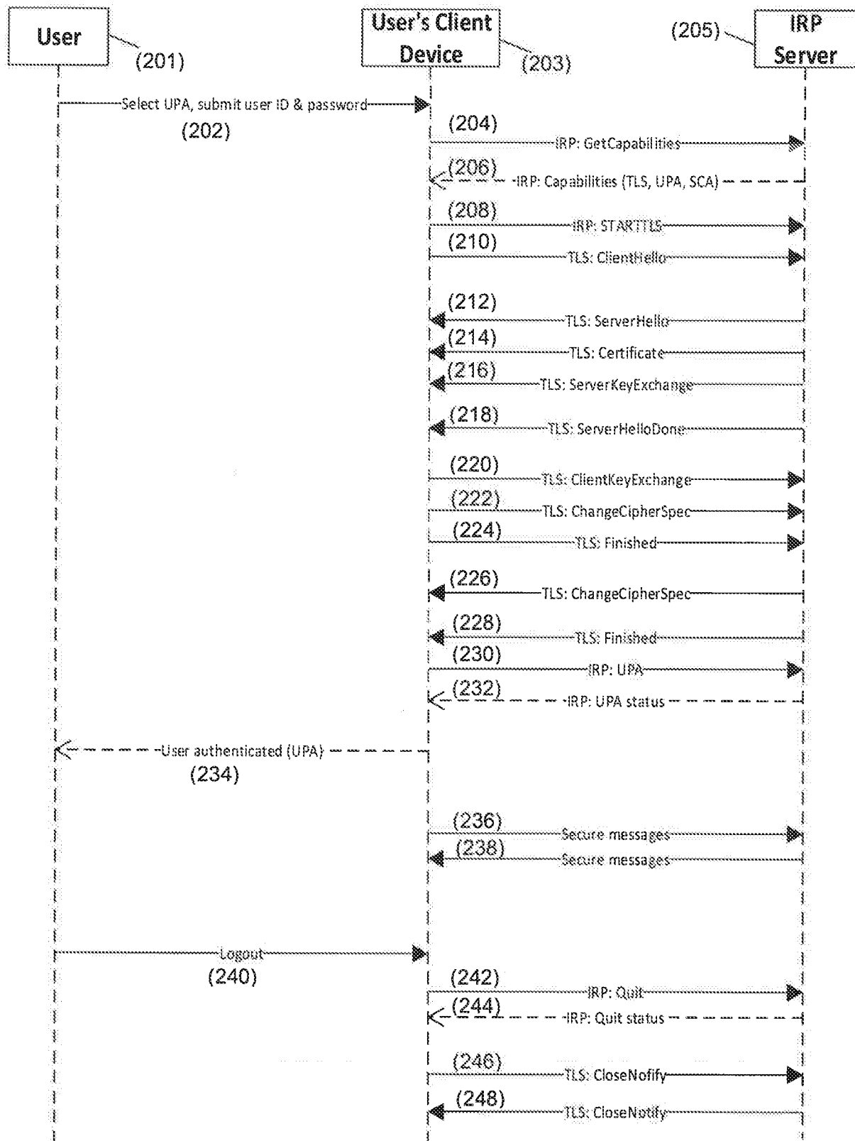
UPA – TLS 1.2 with Server Authentication &amp; Password Authentication
