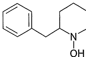
2-benzylpiperidin-1-ol [P6]
