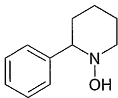
2-phenylpiperidin-1-ol [P5]
