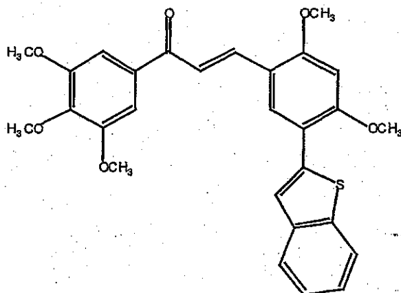
3-[5-(benzo[b]thien-2-yl)-2,4-dimethoxyphenyl]-1-(3,4,5-trimethoxyphenyl)- 2-propen-1-one
