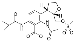
Mixture of cis enantiomers
