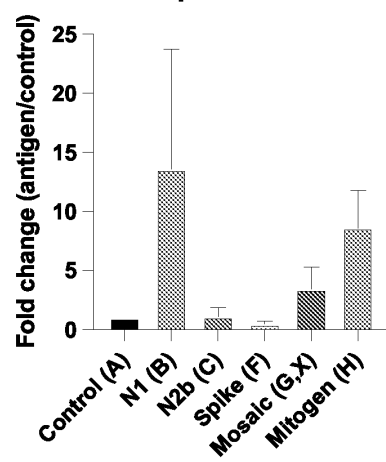
Effect of antigens on IFN \gamma expression in COVID positive individuals
