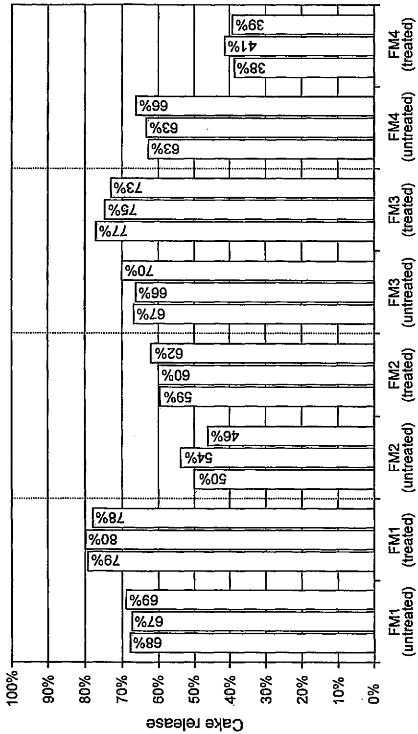
Figure 4 - Cake release results for treated and untreated filtration media
