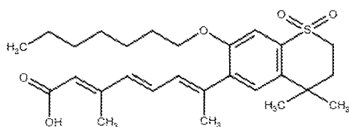
Ro41-5253, or
