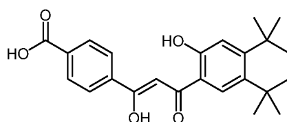
Re 80
