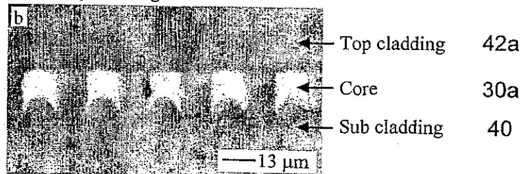
Three-layer waveguides
