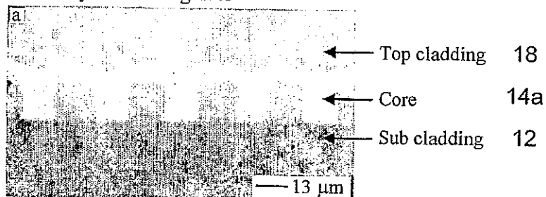
Three-layer rib waveguides
