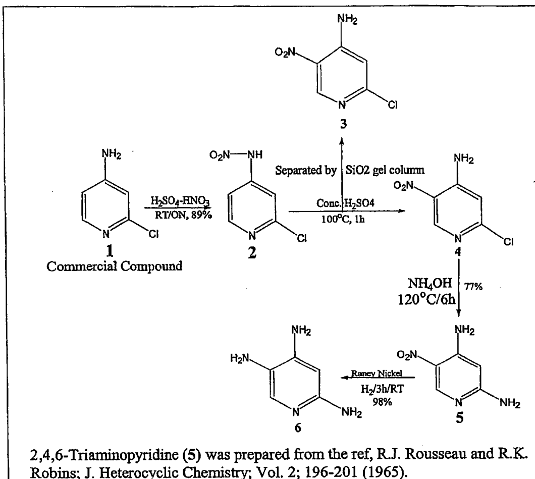
Scheme 37
