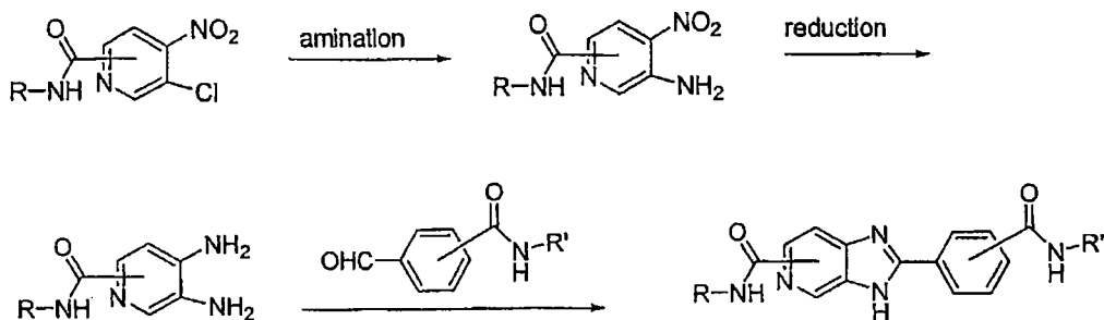
Synthetic Scheme 14
