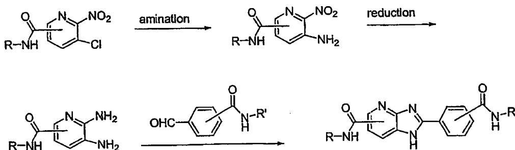
Synthetic Scheme 18
