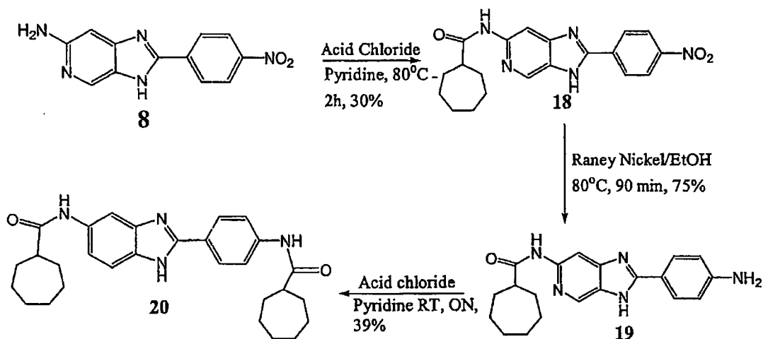
Scheme 40
