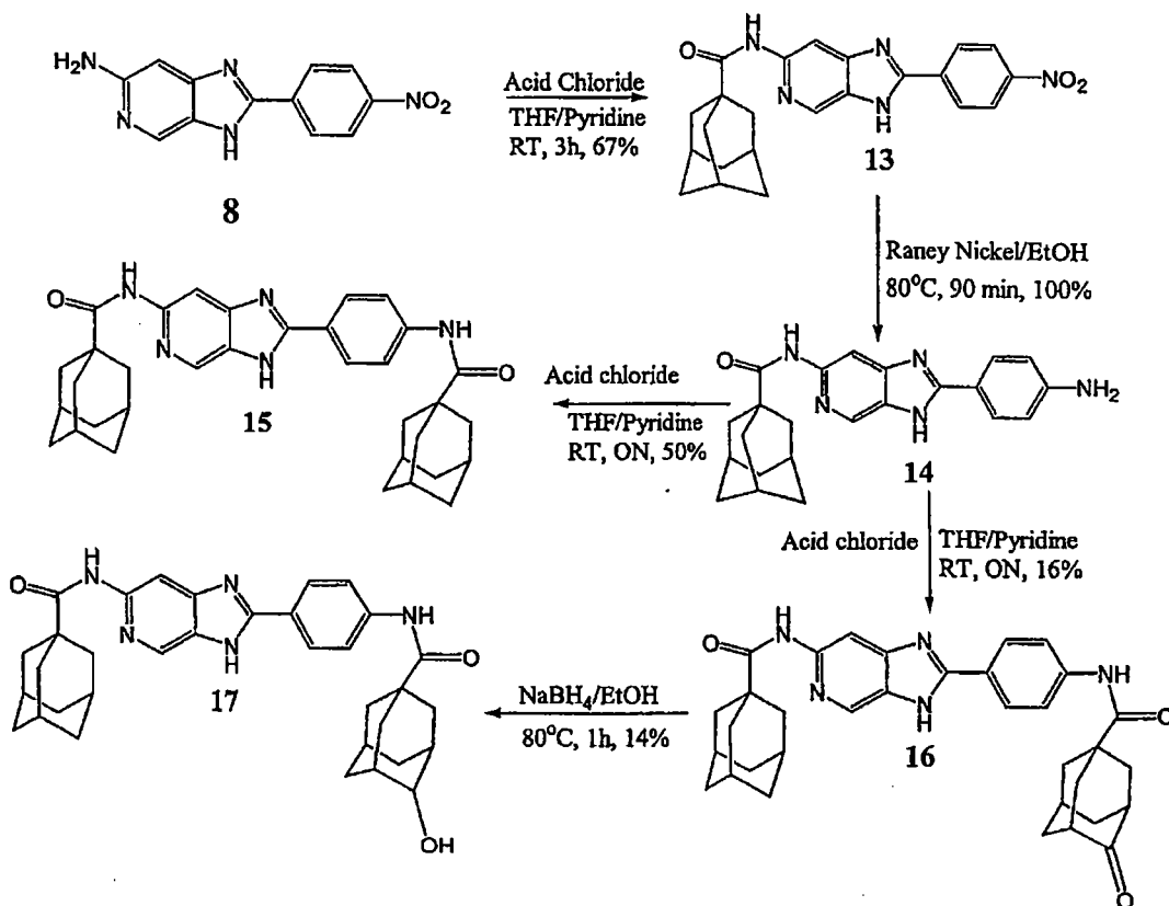
Scheme 39
