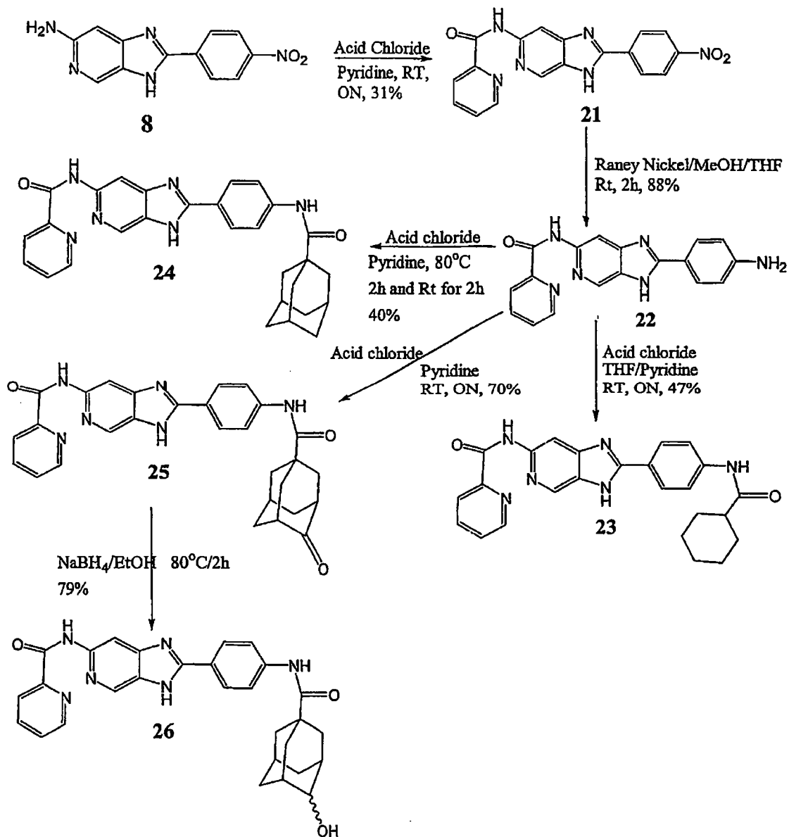
Scheme 41
