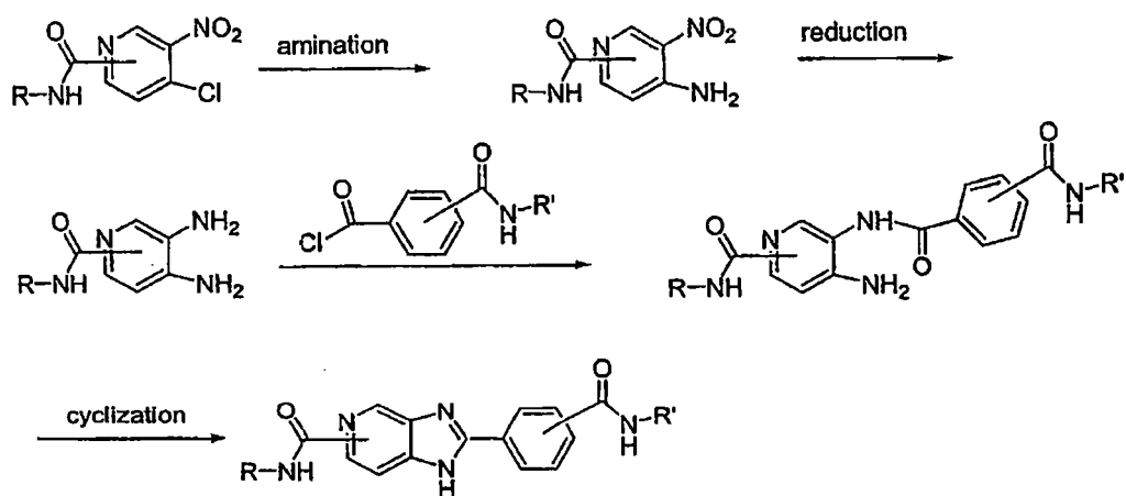
Synthetic Scheme 15
