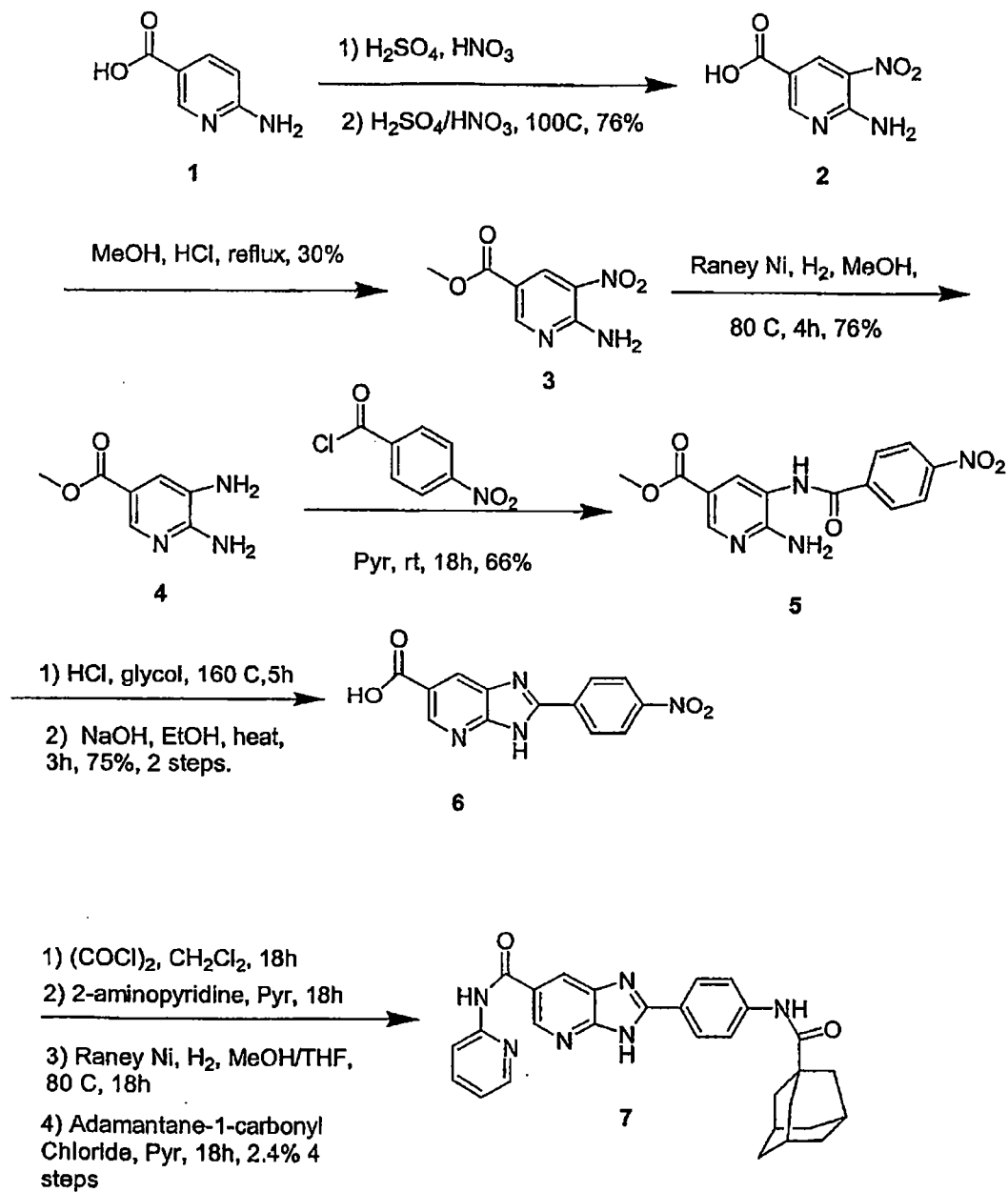
Scheme 42
