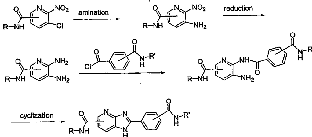
Synthetic Scheme 17
