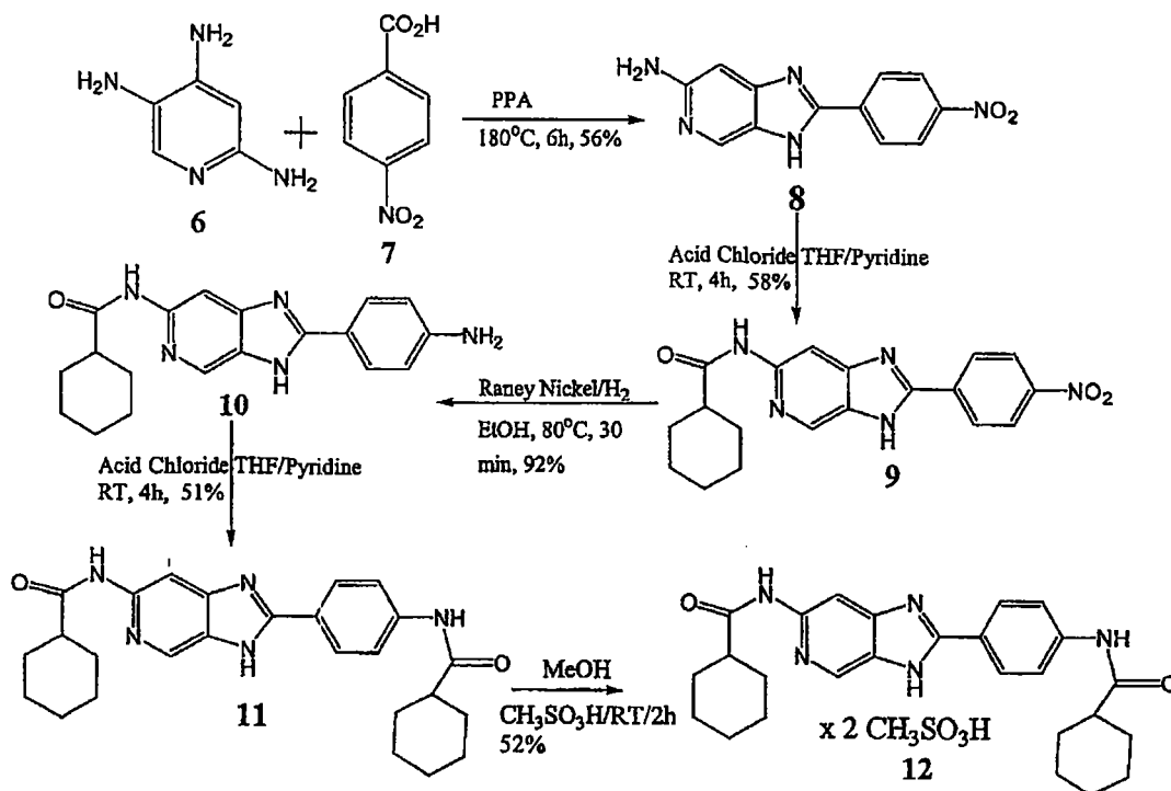
Scheme 38
