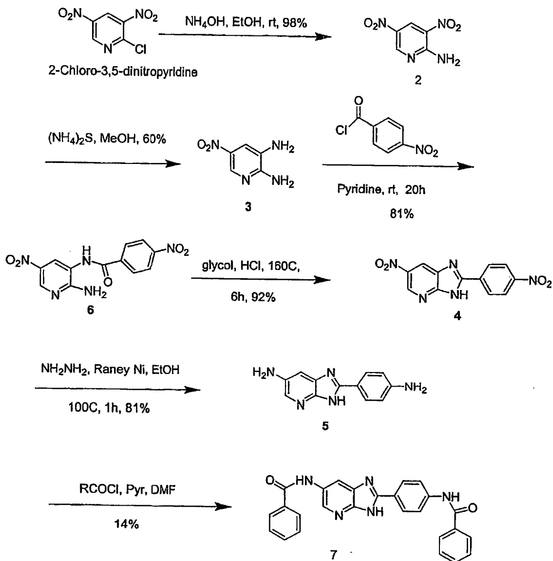
Scheme 36
