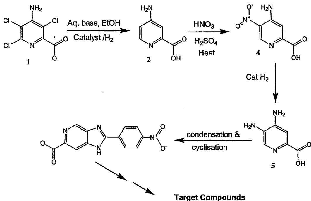
Scheme 44
