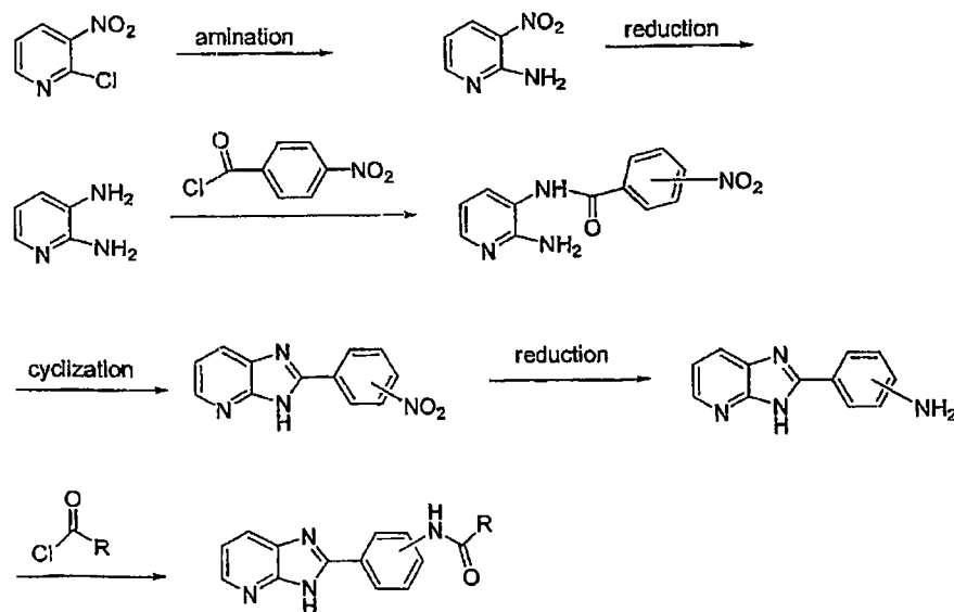
Synthetic Scheme 9
