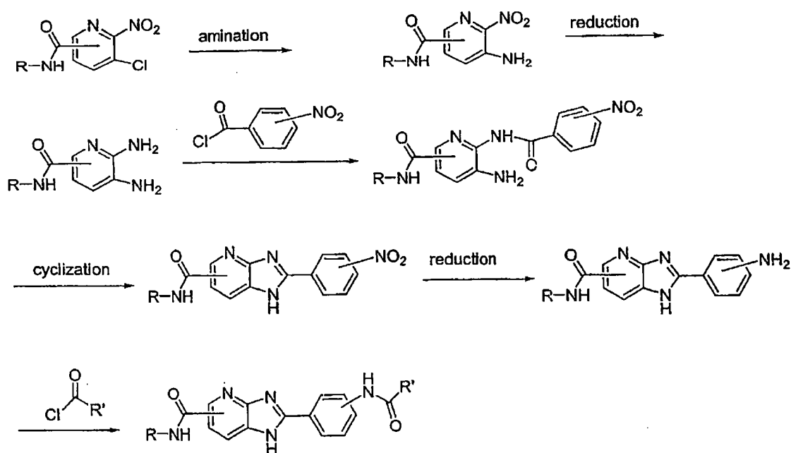
Synthetic Scheme 7
