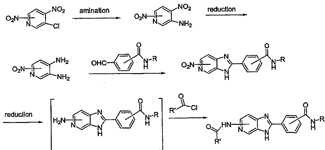
Synthetic Scheme 22
