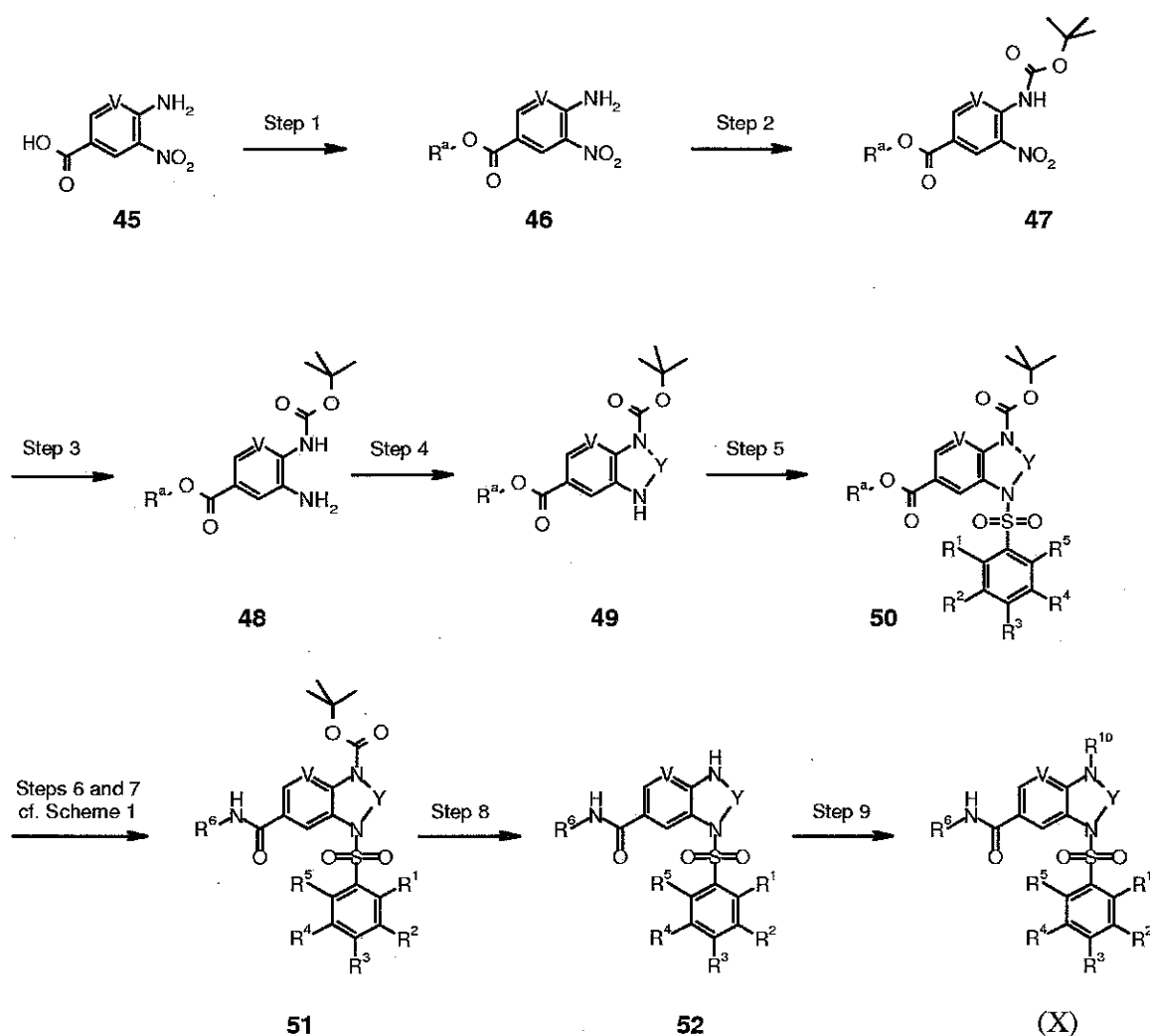
Scheme 12
