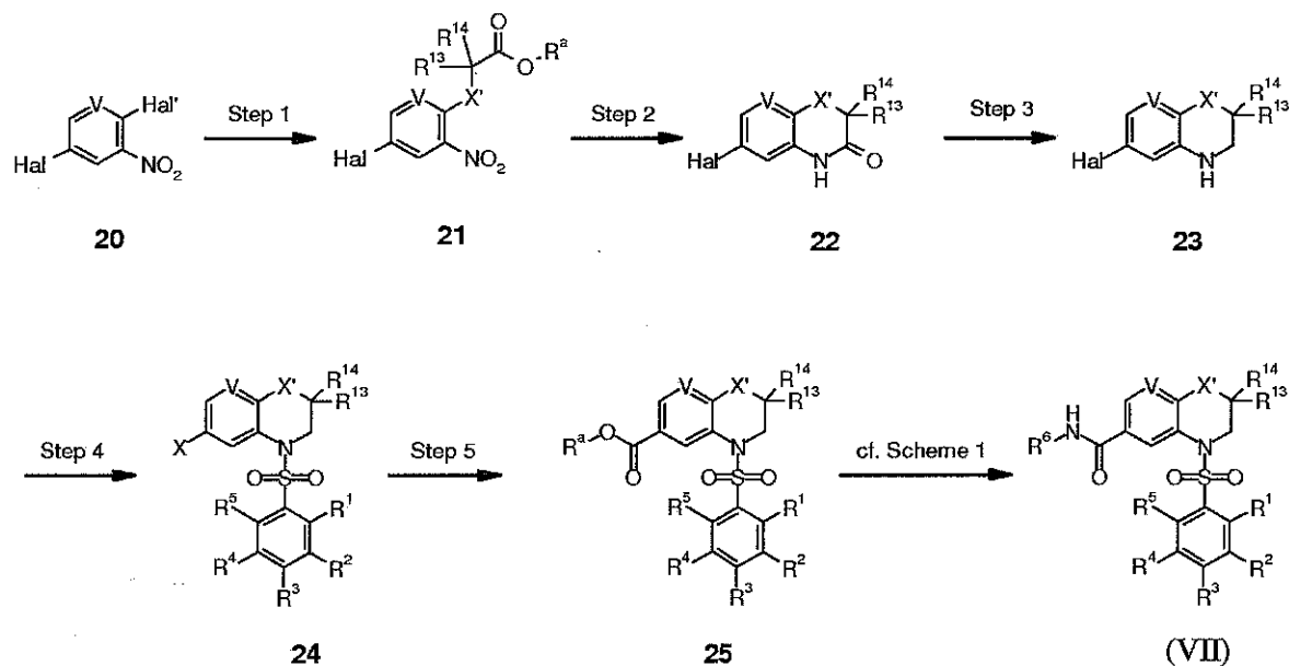
Scheme 7
