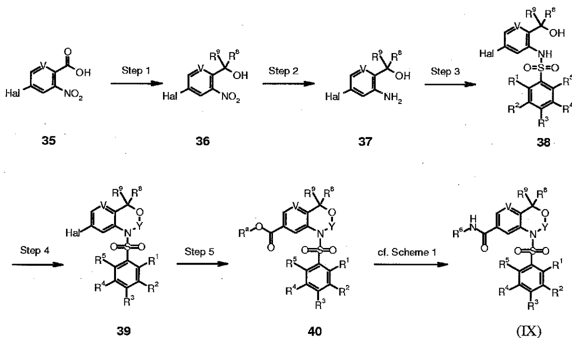
Scheme 10
