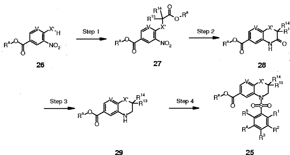
Scheme 8
