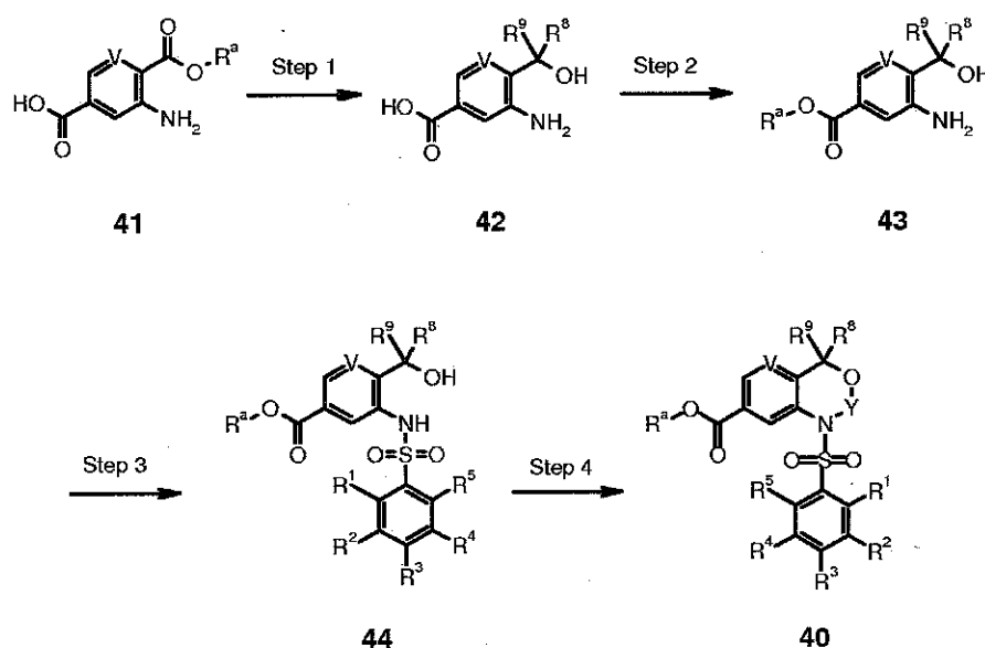
Scheme 11
