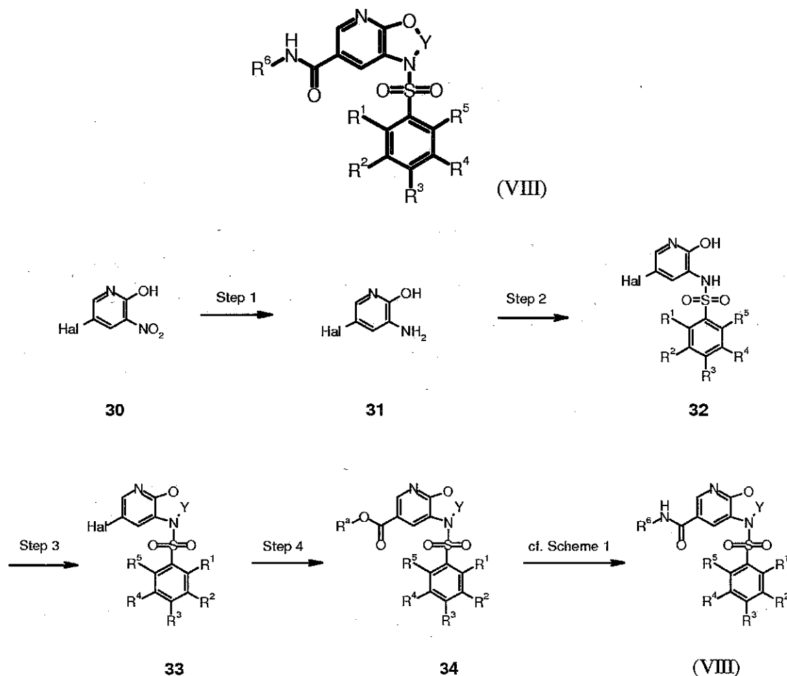
Scheme 9
