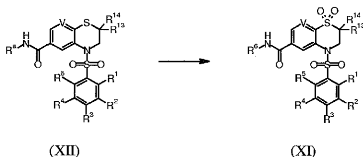
Scheme 13
