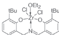
Structure X
