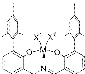
Structure XVIII
