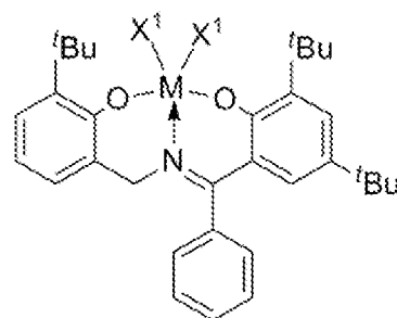
Structure XIX
