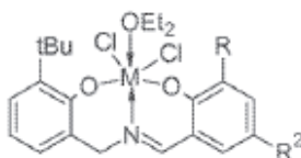
Structure XIV
