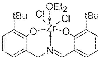
Structure X
