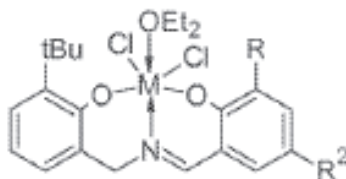
Structure XIV
