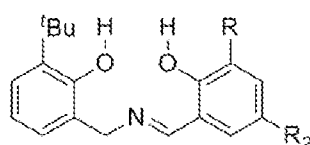
Structure X
