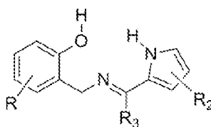
Structure XI
