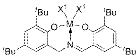
Structure XVI
