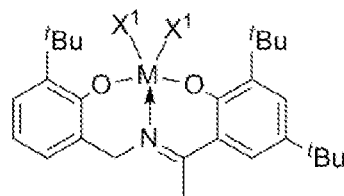
Structure XXI
