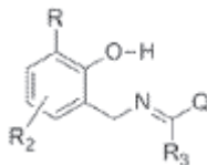
Structure I
