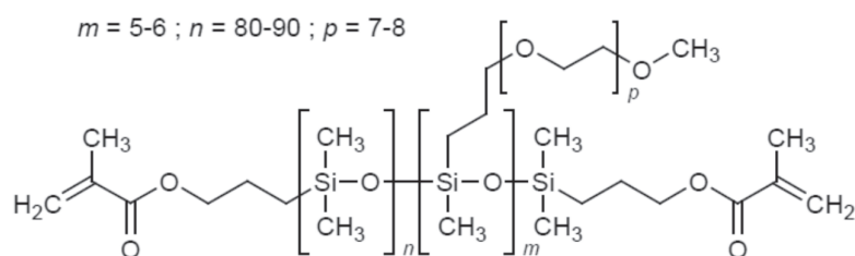
Formula (II)
