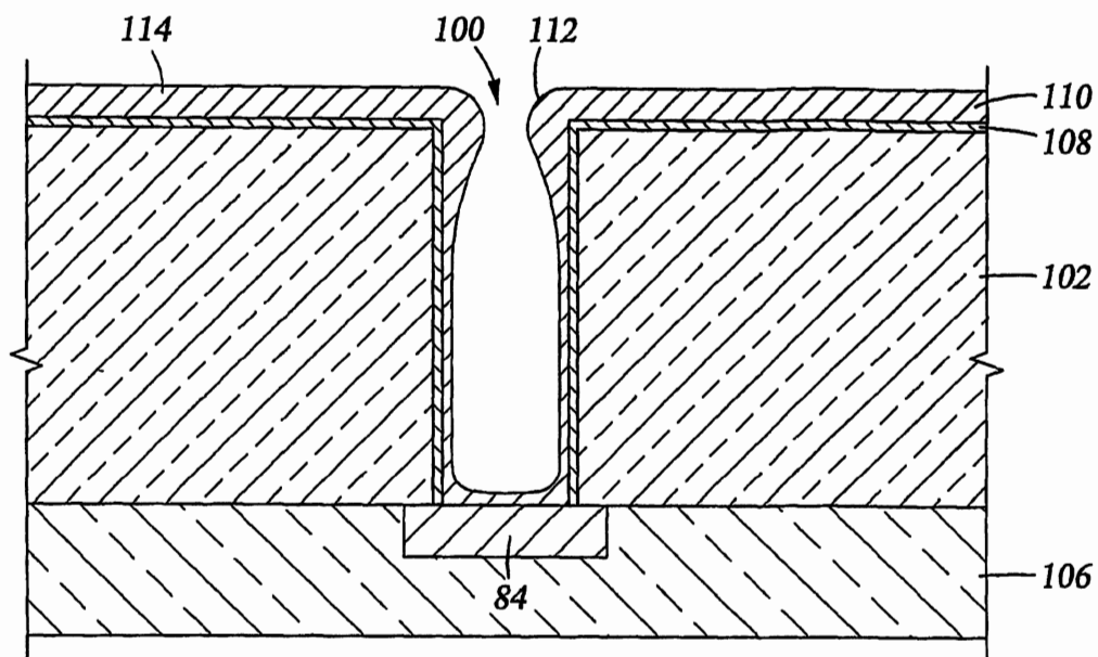
Fig. 4 (PRIOR ART)
