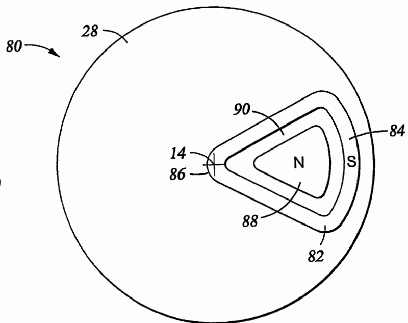
Fig. 3 (PRIOR ART)
