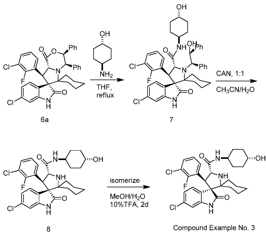
Scheme 9
