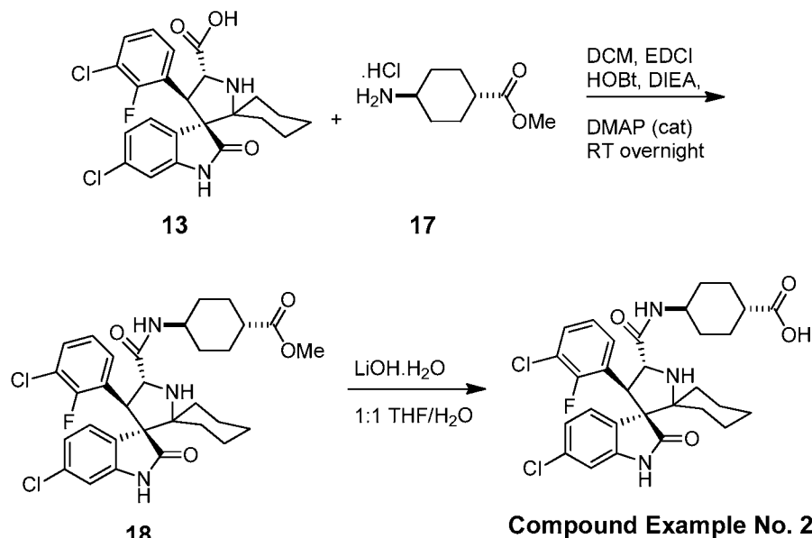
Scheme 13
