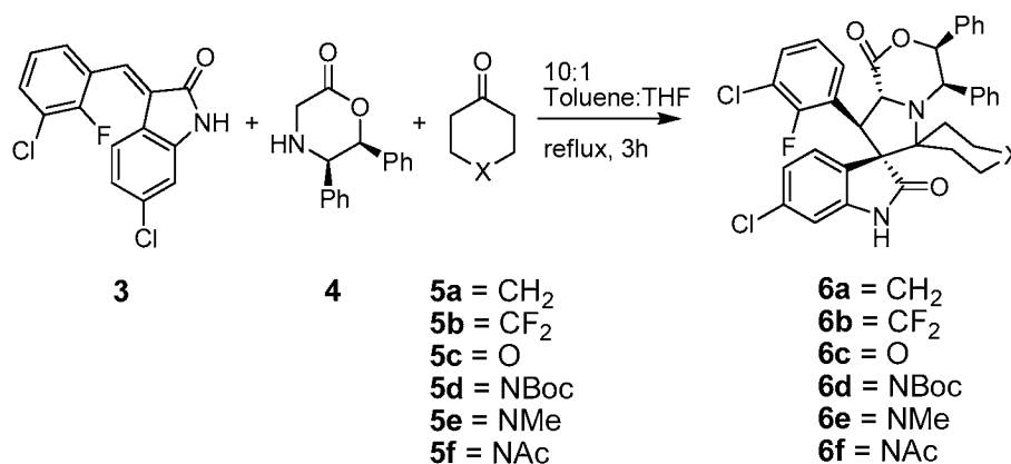
Scheme 8
