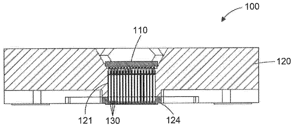
FIG. 1 PRIOR ART
