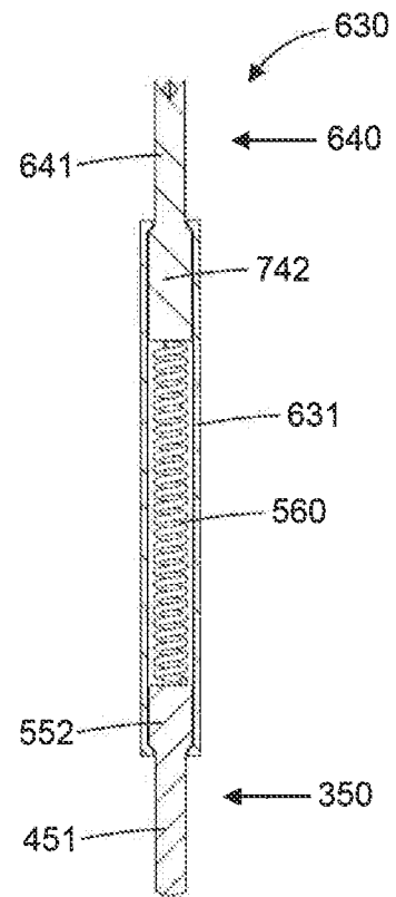
FIG. 7 PRIOR ART
