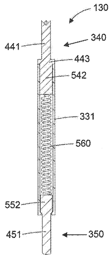
FIG. 5 PRIOR ART
