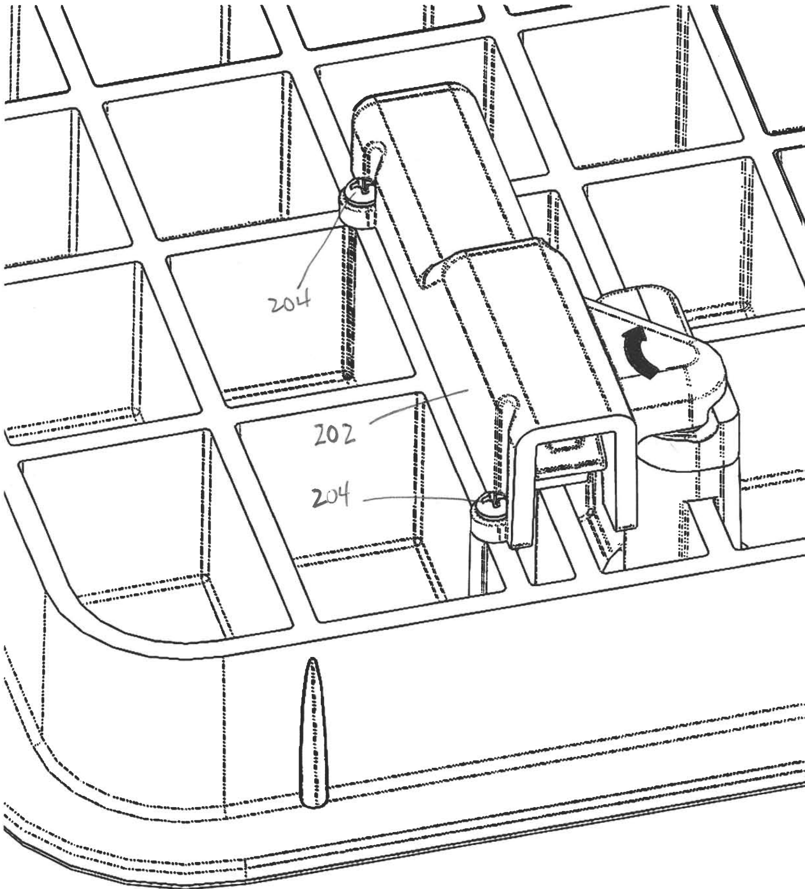
ROTATION OF L-BOLT RETRACTS SLIDE
