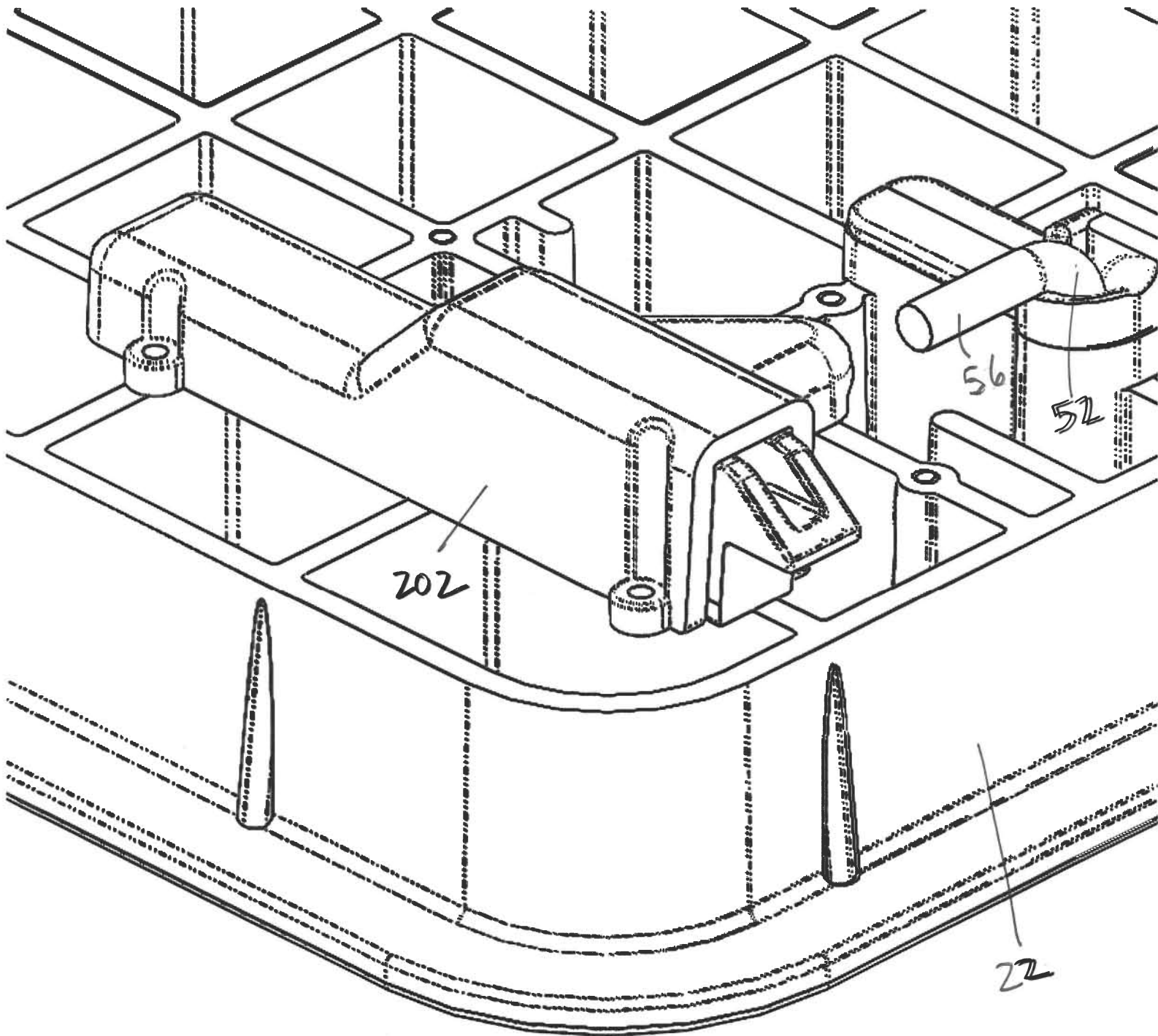
SLAM LATCH ASSEMBLY POSITIONED ON LID, IN LINE WITH L-BOLT
