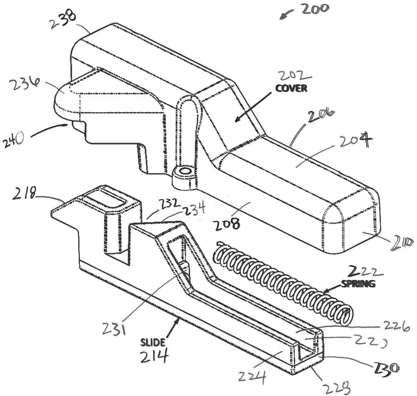
SLAM LATCH COMPONENTS
