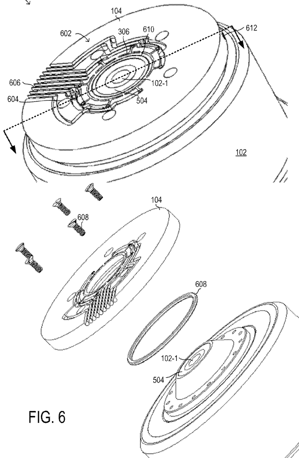
600 ASSEMBLY OF A SENSOR RING MOUNTED TO A MICROSCOPE OBJECTIVE
