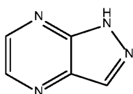
1H-pyrazolo[4,3-b]pyrazine
