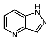
pyrazolo[4,3-d]pyridine (pyrazolo[4,3-d]pyridinyl)
