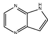
5H-pyrrolo[3,2-b]pyrazine
