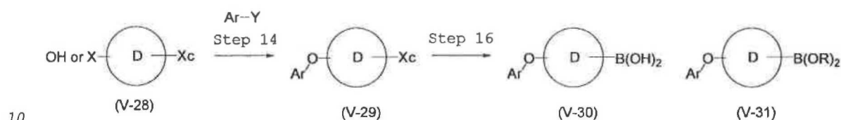
Reaction scheme 10
