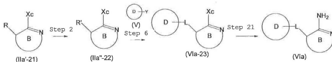
Reaction Scheme 8
