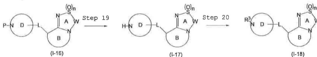
Reaction scheme 6
