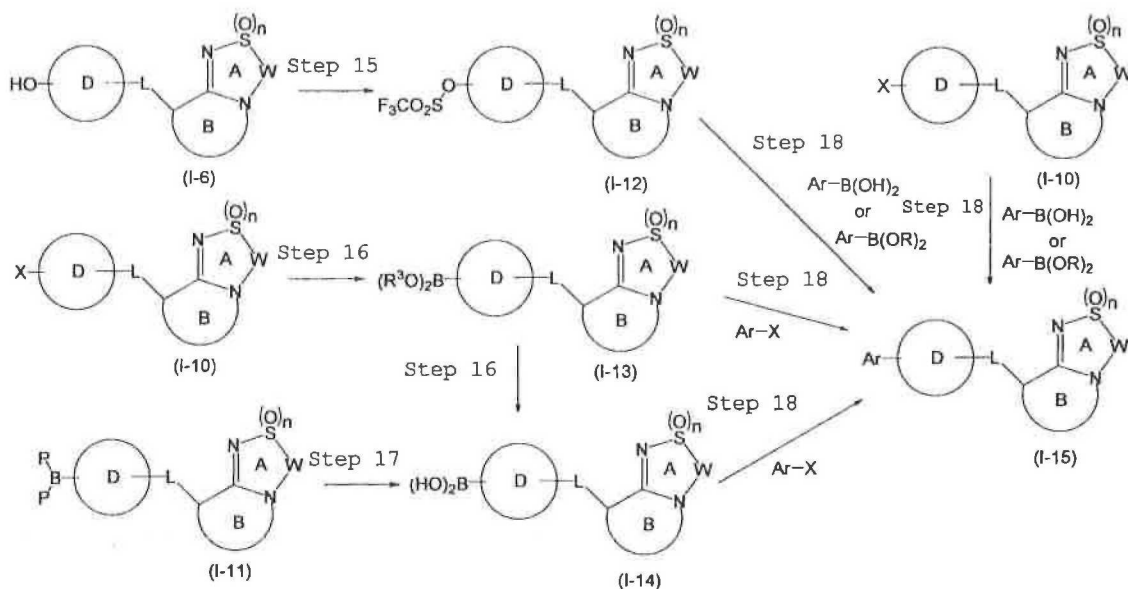
Reaction scheme 5
