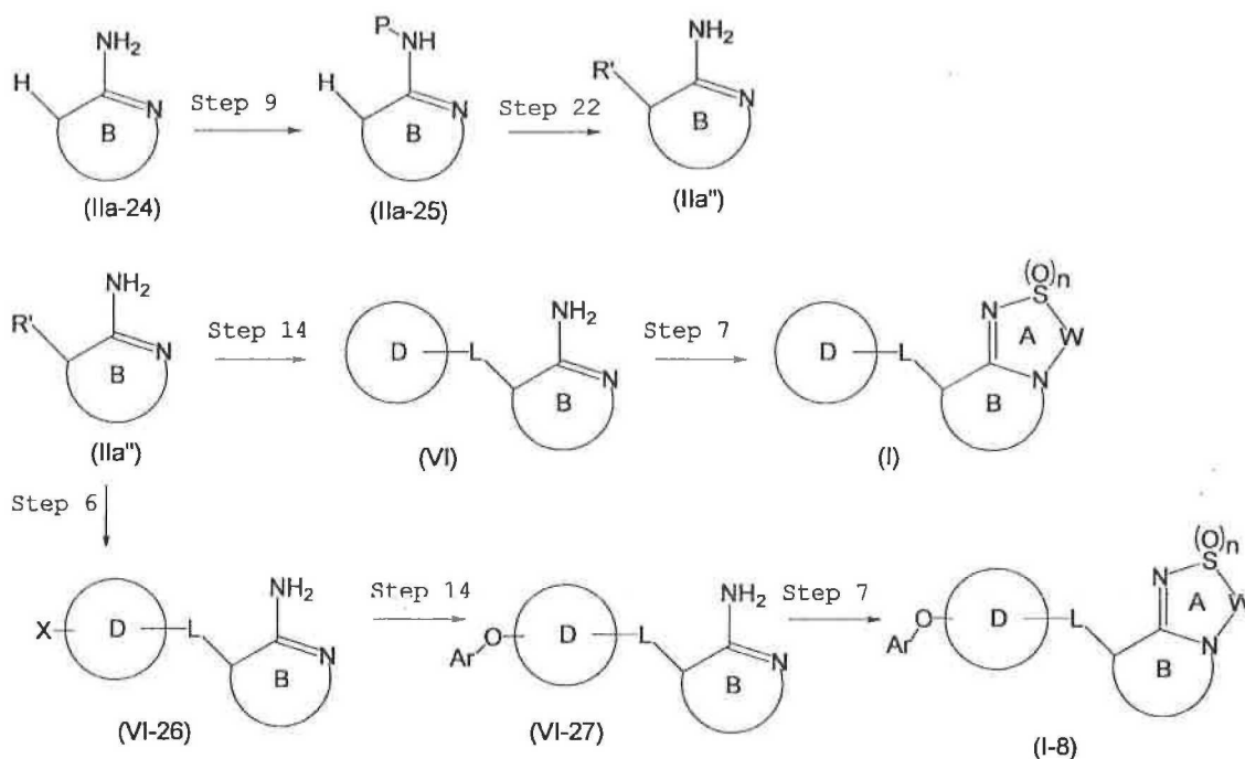
Reaction scheme 9
