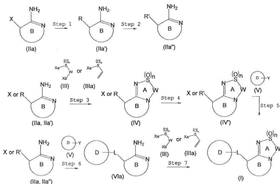
15 Reaction Scheme 1
