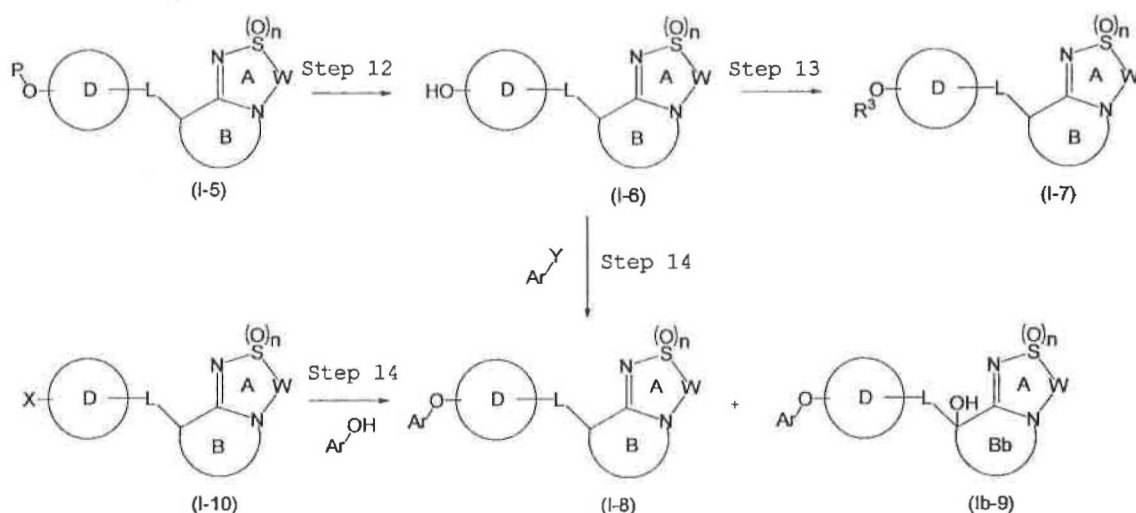
Reaction Scheme 4
