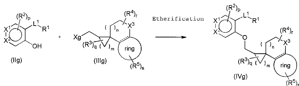
Reaction scheme (Ig)
