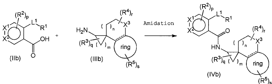
Reaction scheme (Ib)
