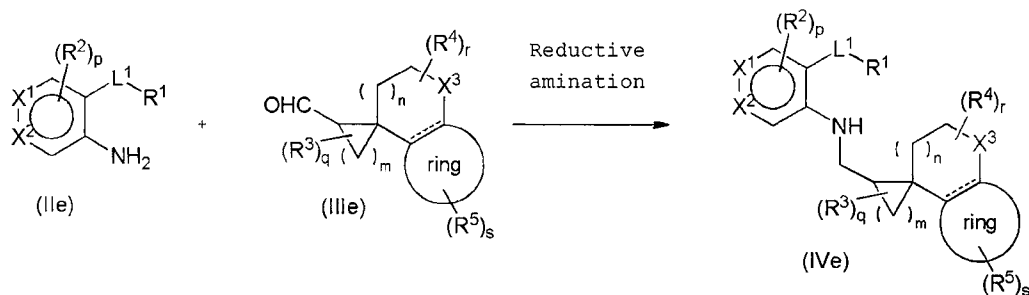
Reaction scheme (Ie)
