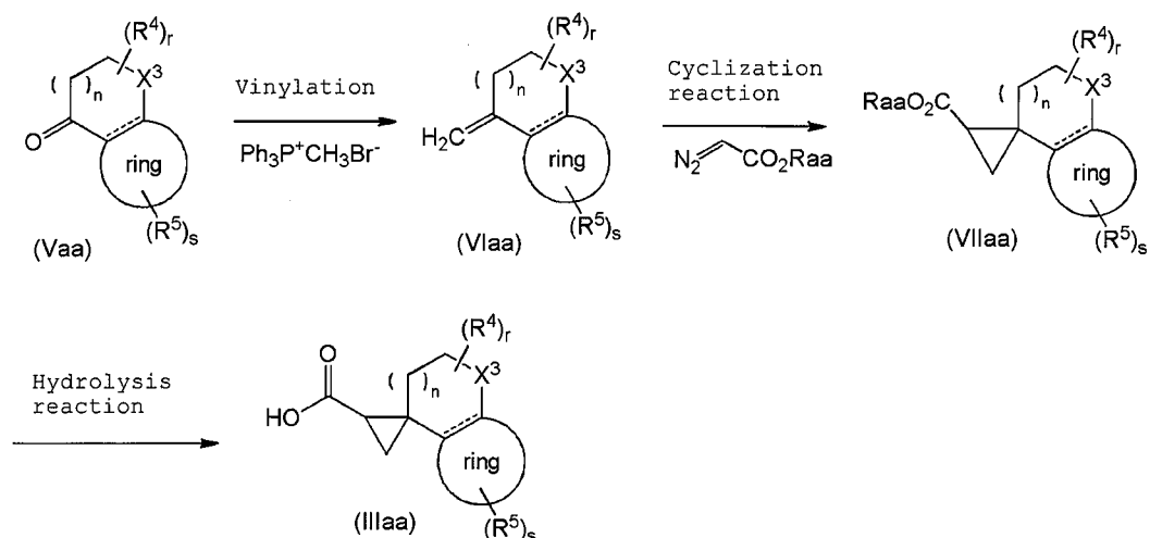
Reaction scheme (Iaa)
