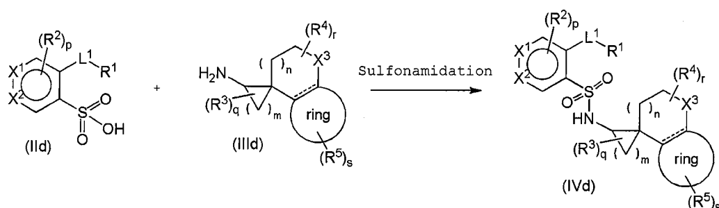
Reaction scheme (Id)
