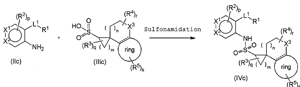
Reaction scheme (Ic)
