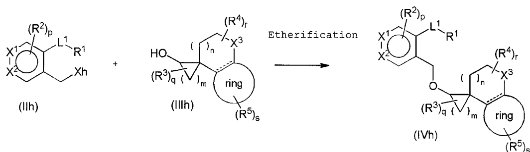
Reaction scheme (Ih)
