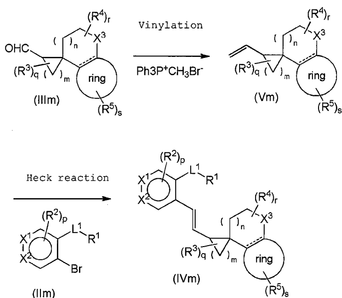
Reaction scheme (Im)
