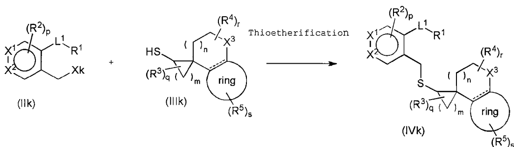
Reaction scheme (Ik)
