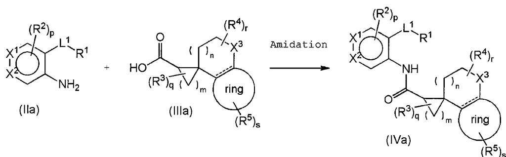
Reaction scheme (Ia)
