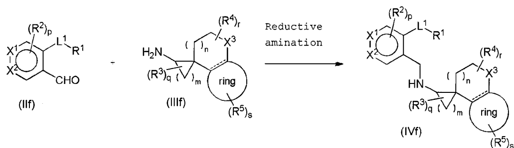
Reaction scheme (If)
