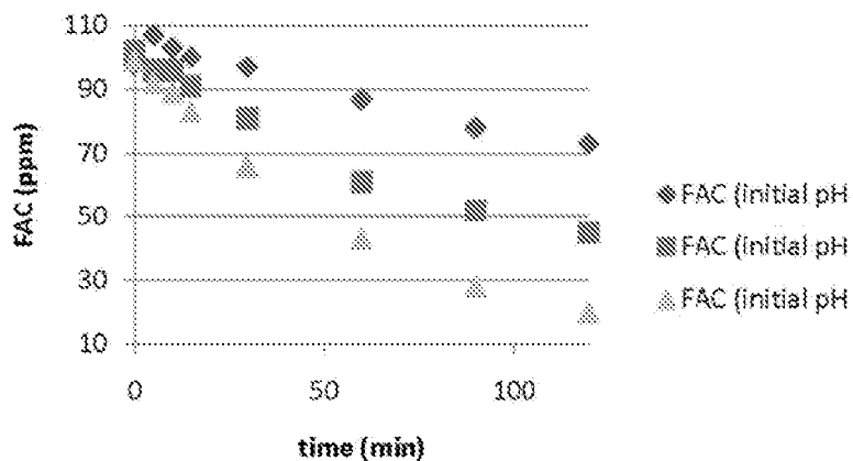
Irradiation of 100 ppm MOS with 365 nm UV
