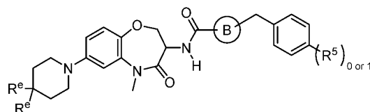
Formula III
