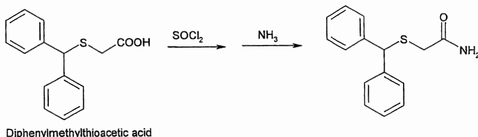
Scheme 7
