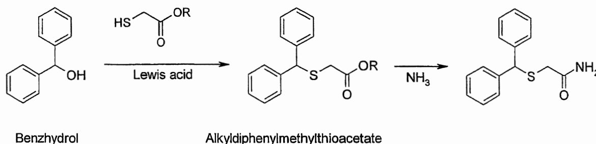
Scheme 3
