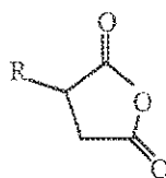
Formula (III)
