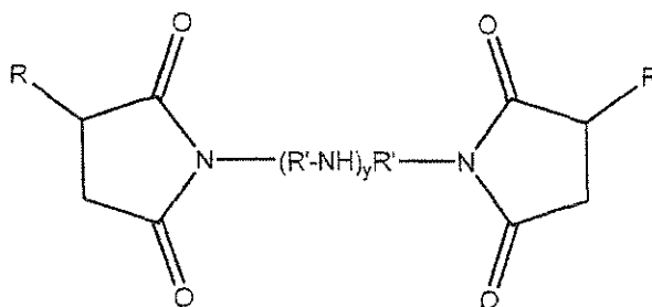
Formula (II)
