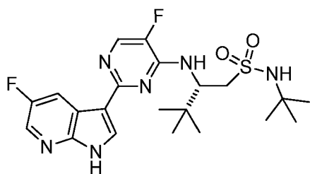
(S)-2-(5-Fluoro-2-(5-fluoro-1H-pyrrolo[2,3-b]pyridin-3-yl)pyrimidin-4-ylamino)-N-tert-butyl-3,3-dimethyl-N-propylbutane-1-sulfonamide (40)
