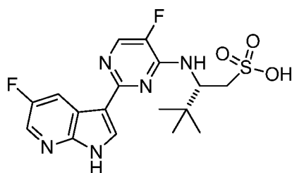
(S)-2-(5-fluoro-2-(5-fluoro-1H-pyrrolo[2,3-b]pyridin-3-yl)pyrimidin-4-ylamino)-3,3-dimethylbutane-1-sulfonic acid (11)
