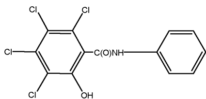
tetrachlorosalicylanilide
