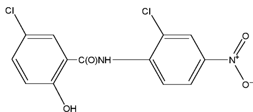
niclosamide
