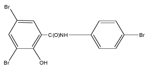
tribromosalalan
