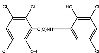
oxyclosanide
