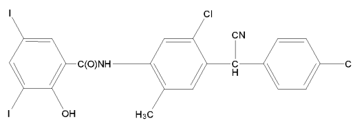
closantel
