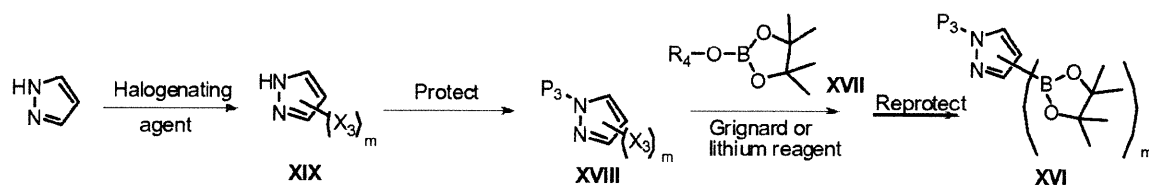
Scheme 14
