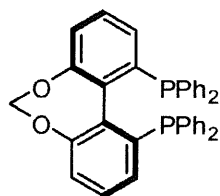
(S)-C1-TunePhos
