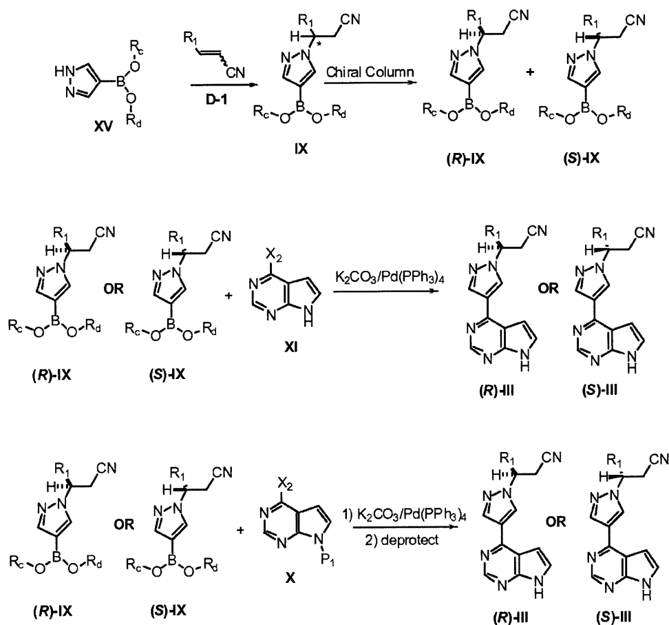
Scheme 5
