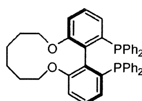
(S)-C6-TunePhos
