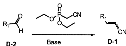
Scheme 9
