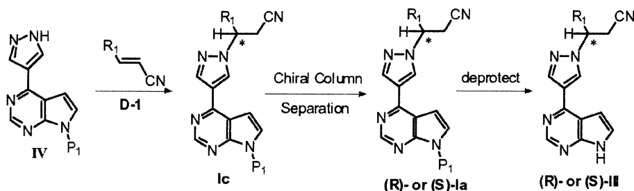
Scheme 6
