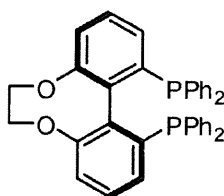
(S)-C2-TunePhos
