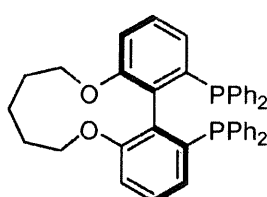
(S)-C5-TunePhos
