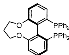
(S)-C3-TunePhos
