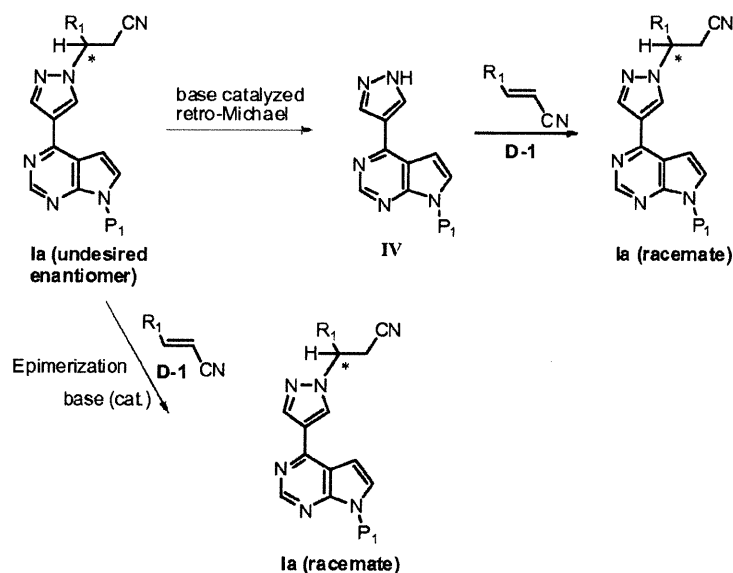
Scheme 8
