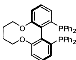
(S)-C4-TunePhos
