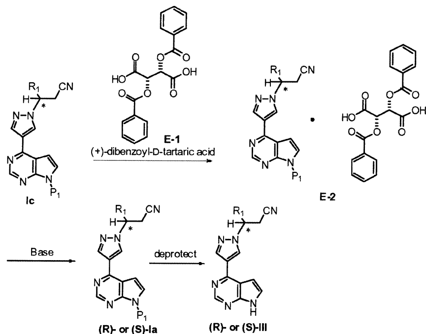
Scheme 7
