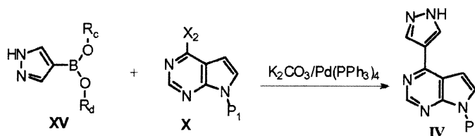
Scheme 10
