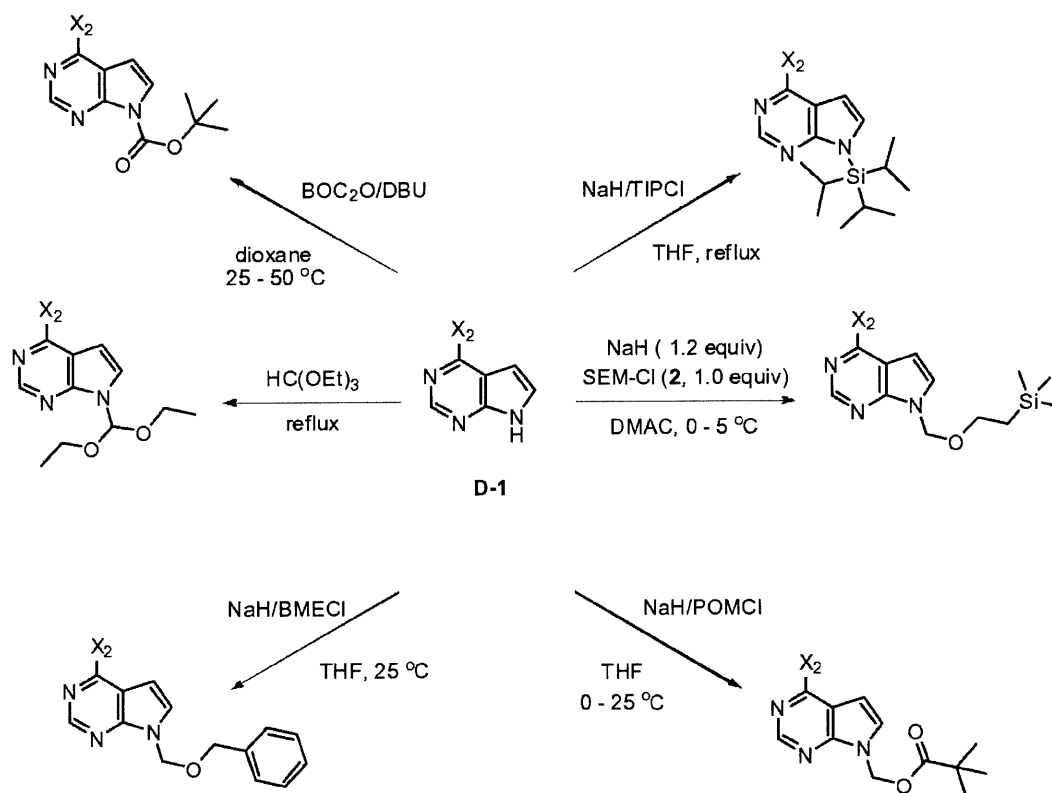
Scheme 13
