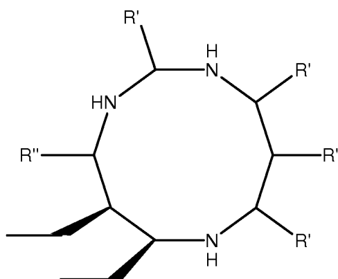
10 substituted 1,5,9 triazacyclodecane
