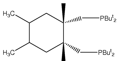
cis-1, 2-bis (di- tert -butylphosphinomethyl), 1, 2, 4, 5 tetramethylcyclohexane
