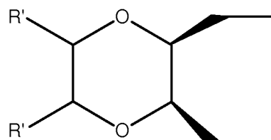
5 and/or 6 substituted 1,4 dioxane
