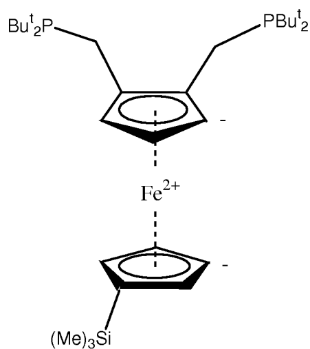
1,2-bis(di-tert-butylphosphinomethyl)-1'-trimethylsilyl ferrocene
