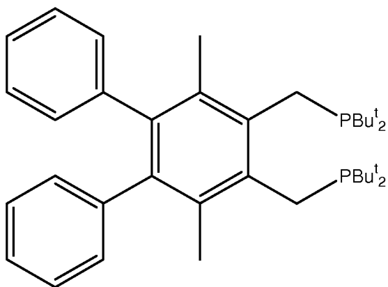
1,2-bis(di-tert-butyl(phosphinomethyl))-4-phenyl benzene
