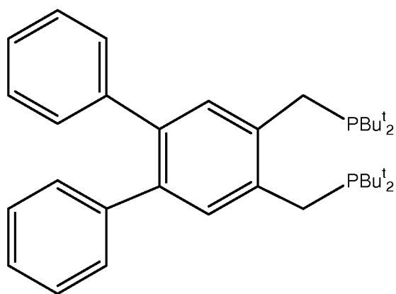
10 1,2bis(di-tert-butyl(phosphinomethyl))-4,5-diphenyl benzene
