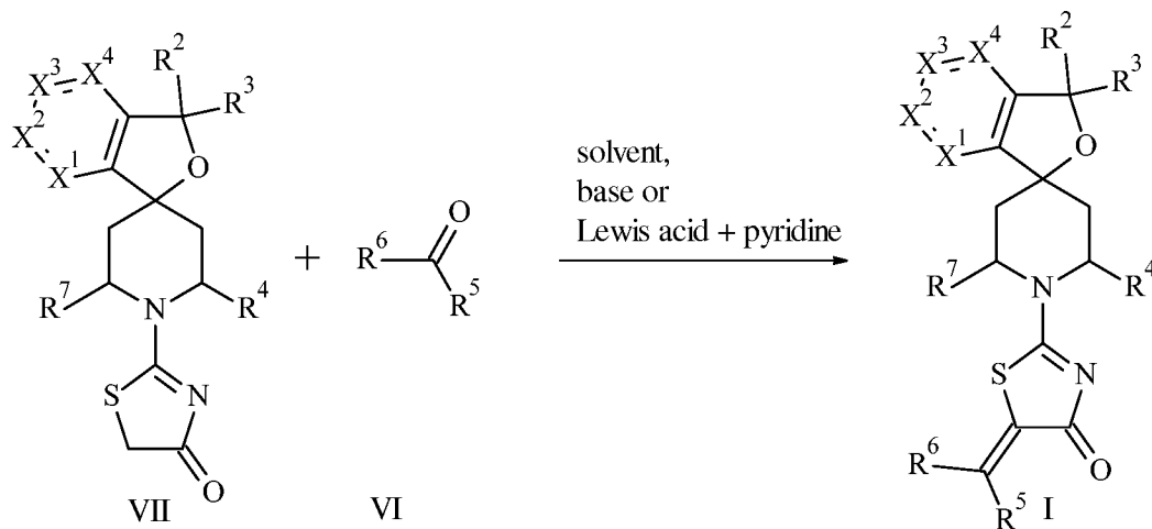
Scheme 4: General Scheme D
