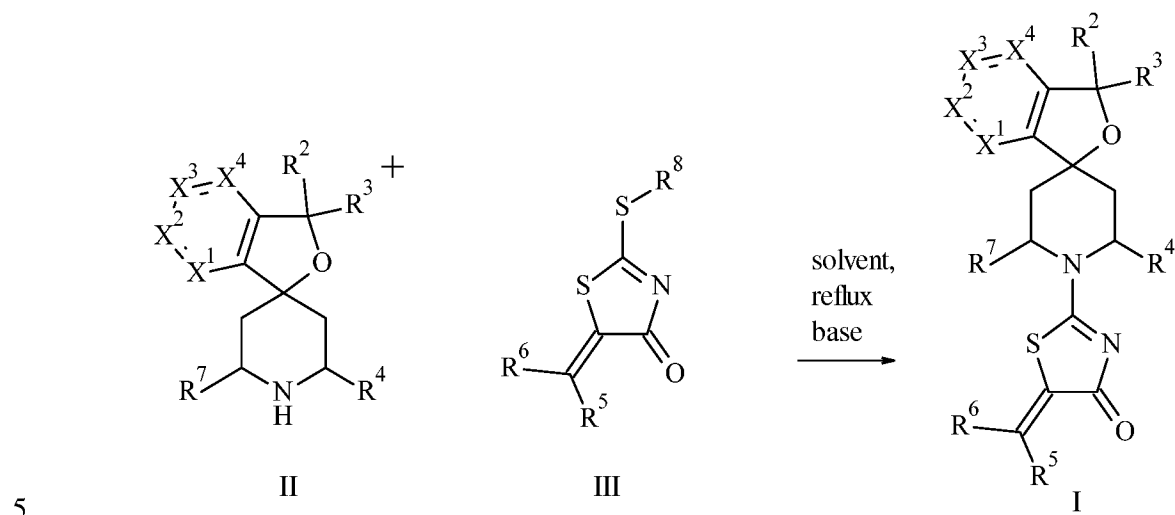
Scheme 1: General Scheme A
