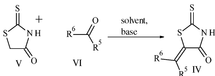
Scheme 3: General Scheme C
