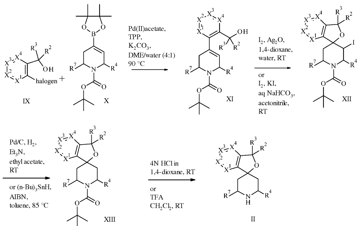
Scheme 13: General Scheme G
