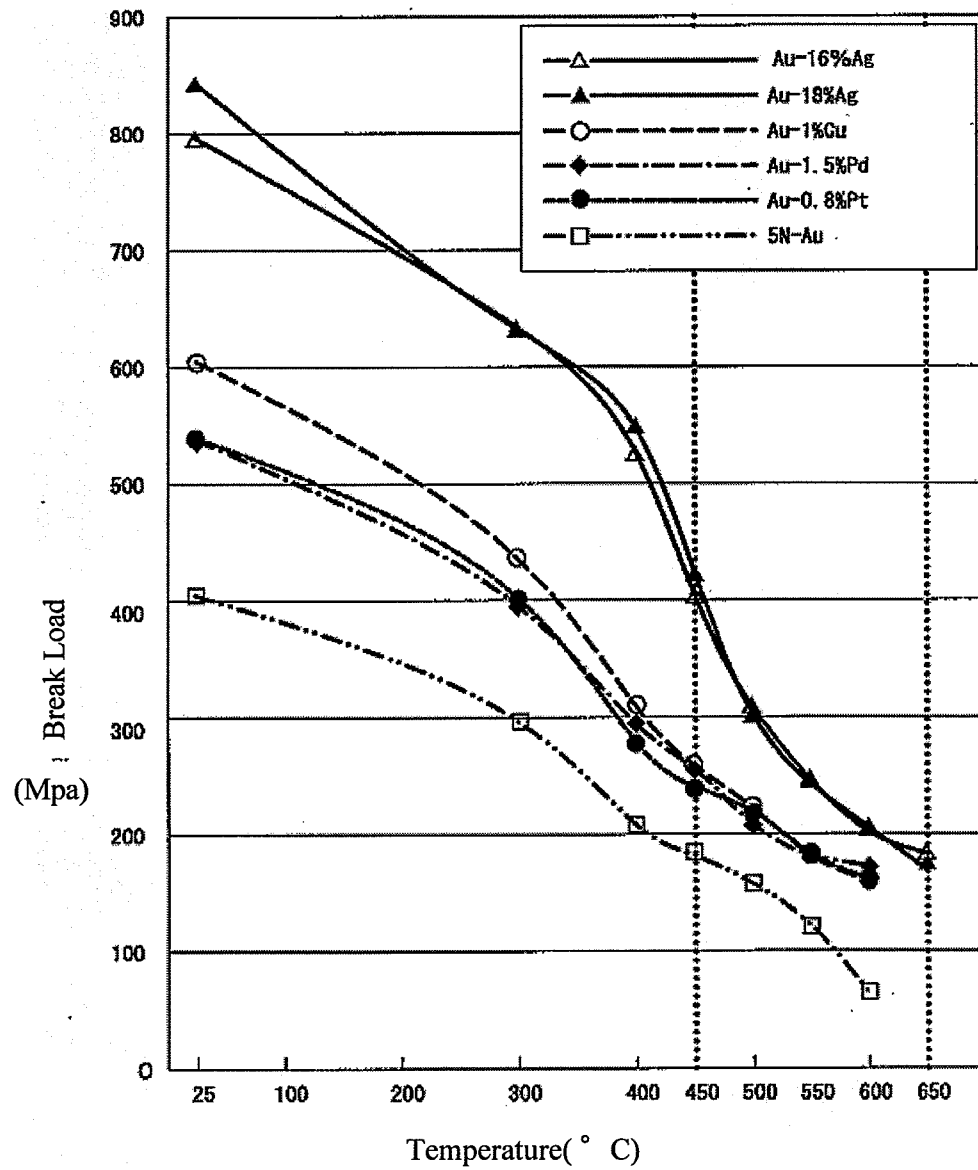
Relation between Heat-treatment temperature and Break Load (BL)
