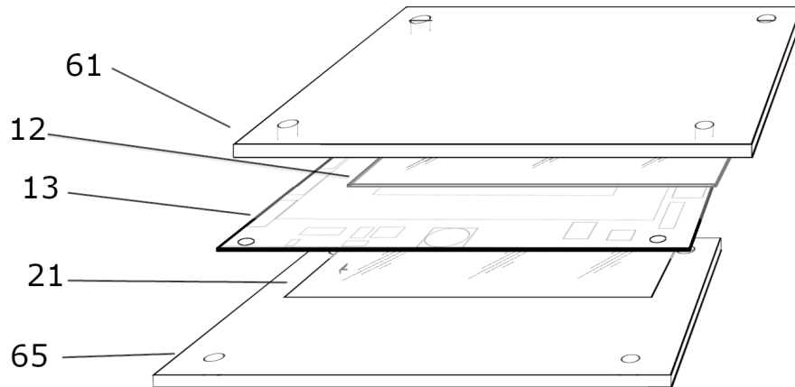
Fig.6 Layered view
