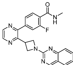
Scheme 3
