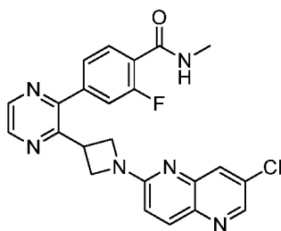
Scheme 7
