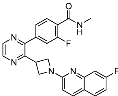
Scheme 4
