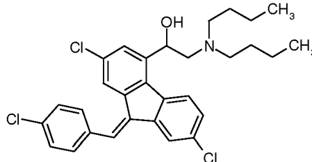
Lumefantrine
