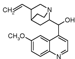
Quinine
