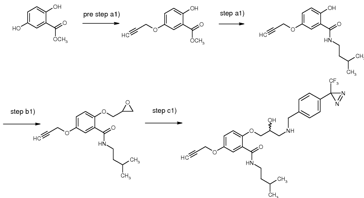
REACTION SCHEME 4
