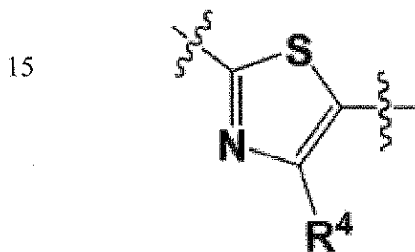
Compound 5
