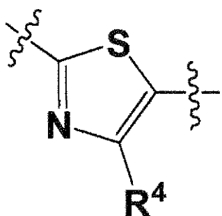
Compound 5
