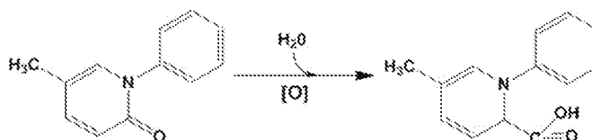
Scheme 1. Pirfenidone hydrolyzed to its non-functional metabolite
