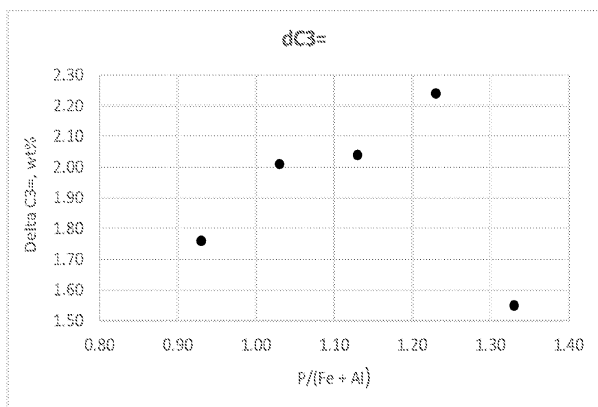
FIG. 2: Propylene make vs P(Fe + Al) molar ratio
