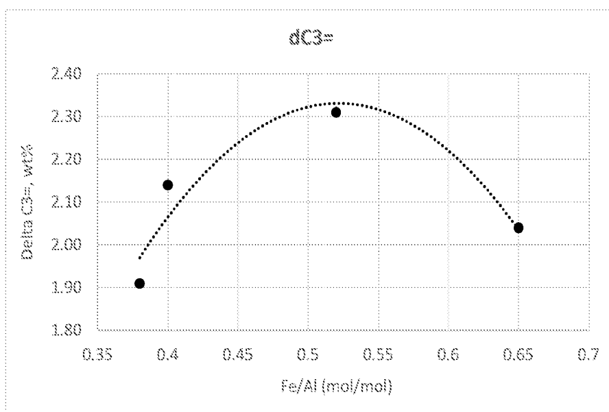
FIGURE 1: Propylene make vs Ratio of Framework Fe:Al
